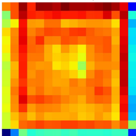
Grad-CAM Heatmap
