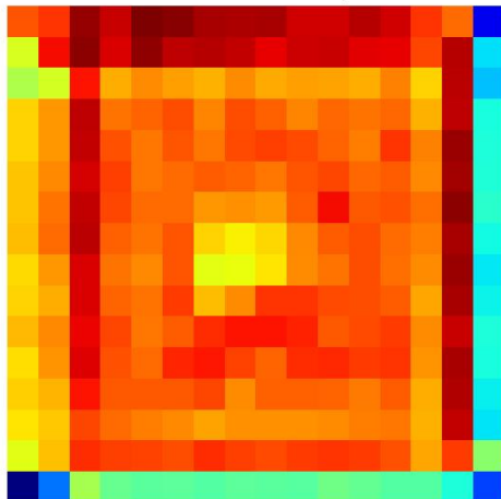
Grad-CAM Heatmap
