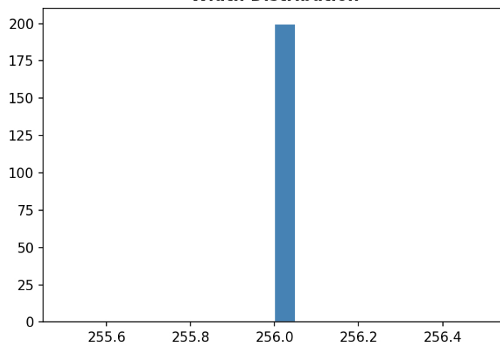
Width Distribution
