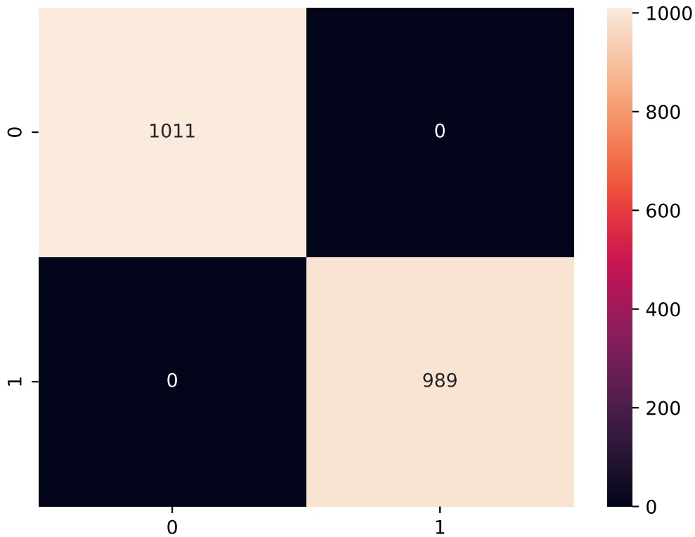
Confusion Matrix (RF)
