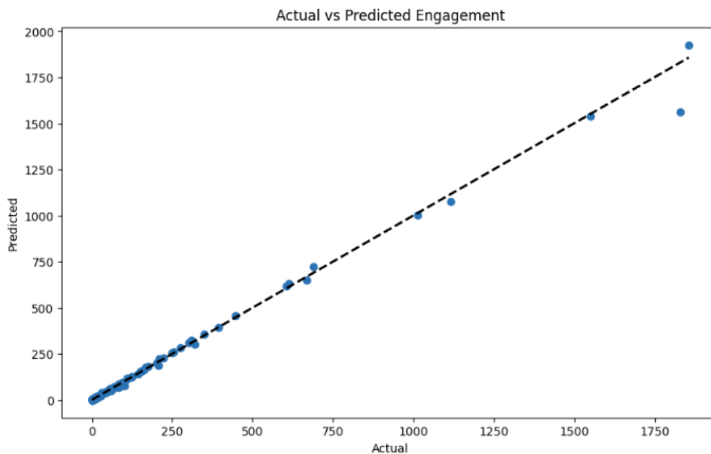
Figure 7: Actual vs Predicted Engagement
