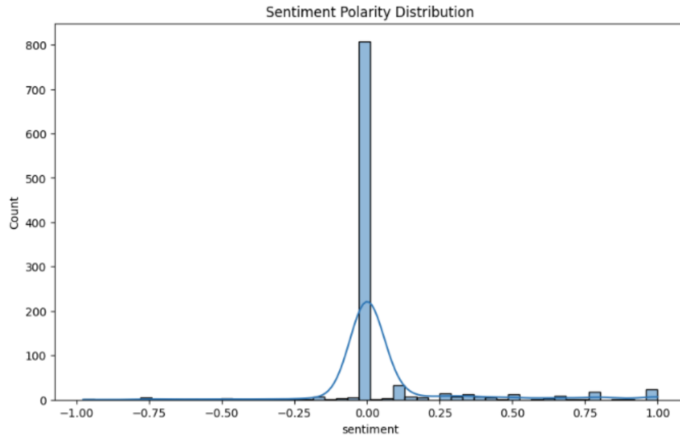
Figure 6: Distribution graph of sentiment polarity
