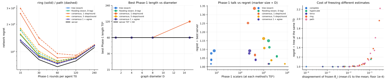
Figure 5: Exploration length and agreement on graphs (E28, N = 16 , 10 paired trials). From left: regret against the Phase-1 length T_0 on the ring and path; the best T_0 barely moves with D ; Phase-1 communication against regret; and the regret cost of agents freezing different estimates, which one agreement pass at the freeze removes.
