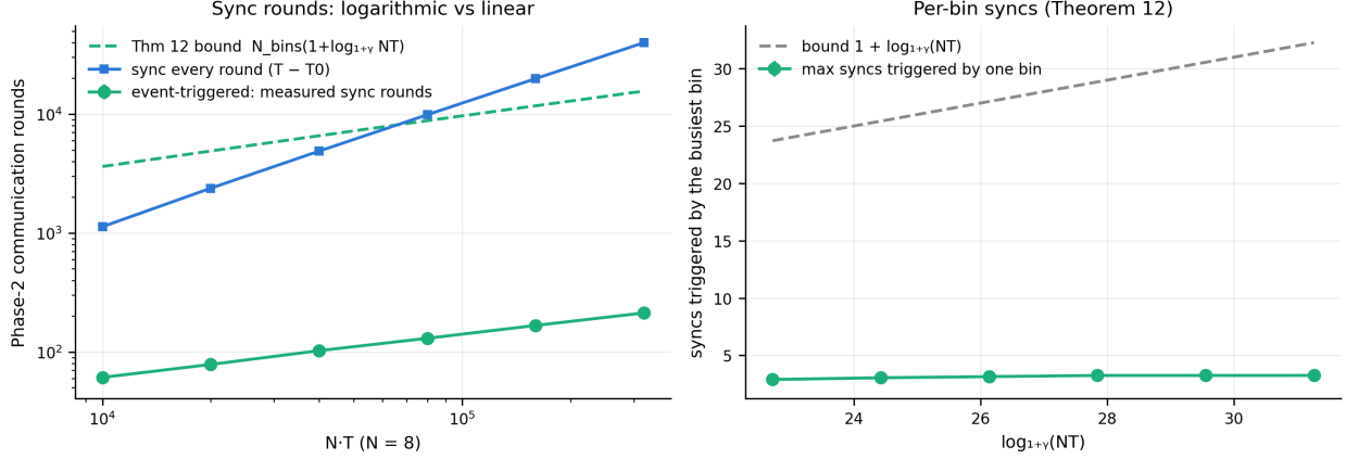
Figure 2: Empirical check of Theorem 12 (E22 part 2, N = 8 ). Left: Phase-2 sync rounds of the event trigger grow logarithmically (61→213 as NT grows 32 \times ) while per-round sync grows linearly; the theorem’s bound (dashed) is 60–75 \times above the measurement. Right: the busiest bin triggers about 3 syncs against a per-bin bound of 24–32.
