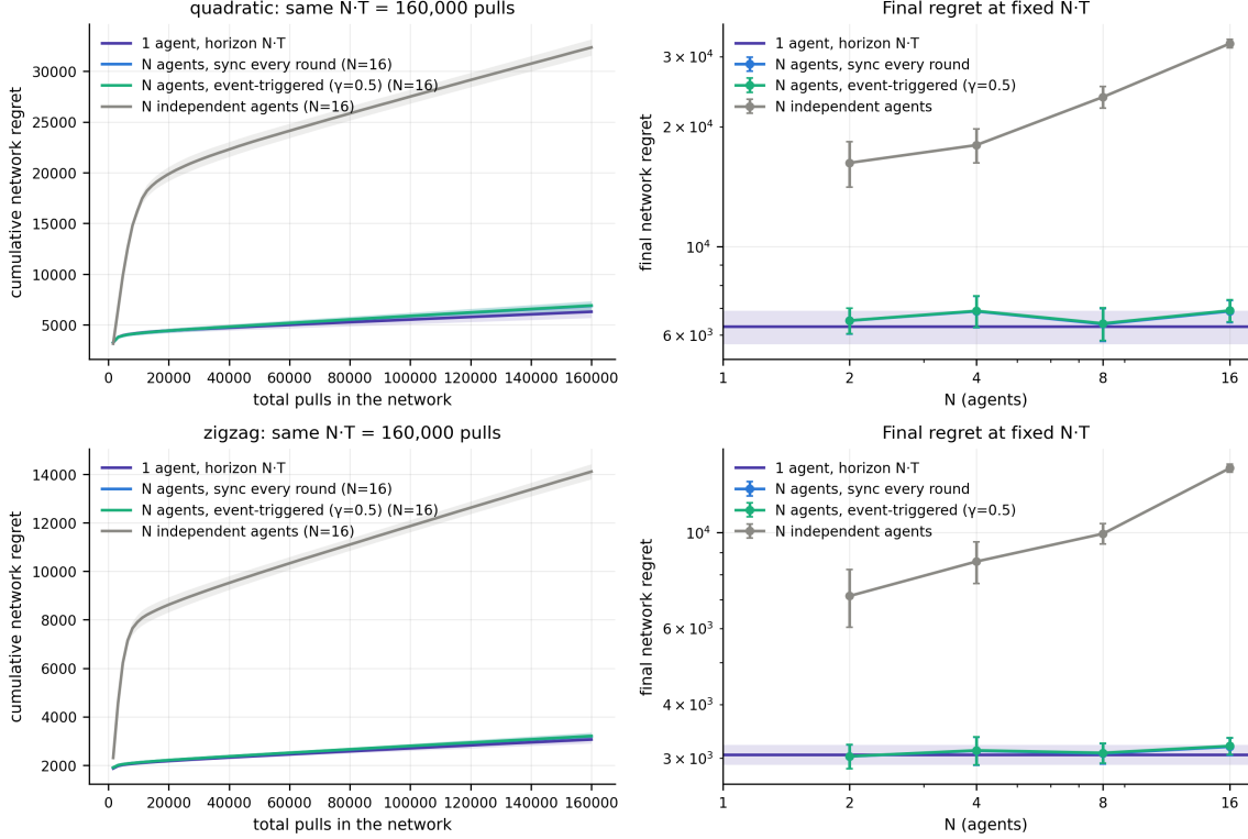
Figure 1: Empirical check of Theorems 3 and 9 (E22, 20 paired trials). Fixed total budget NT = 160000 , same pooled exploration and bin width for every N . Left: regret against total pulls; the single agent at horizon NT and N = 16 synced agents overlap. Right: final regret against N ; synced agents stay within 0–10% of the single agent and never beat it, while independent agents are 2.3\text{--}5.1\times worse.
