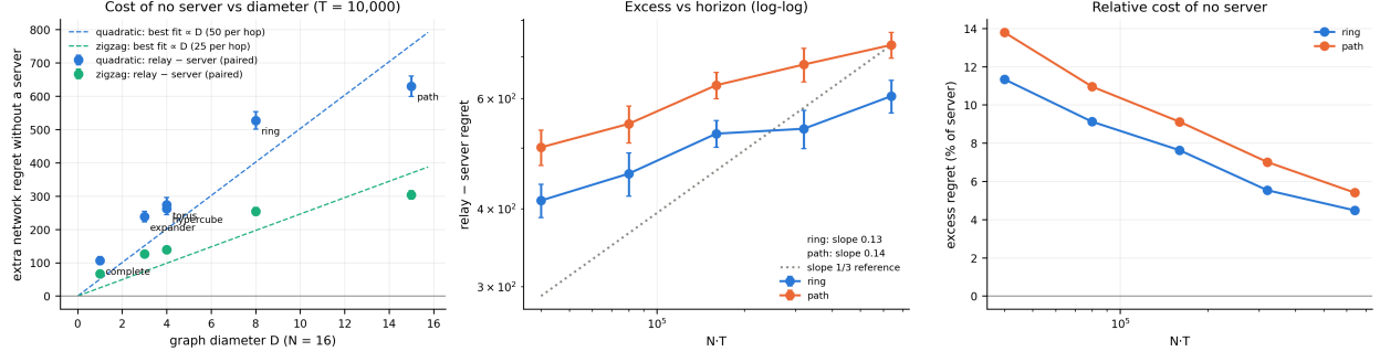
Figure 4: Theorem 16 against measurement (E23, N = 16 , 20 paired trials). Left: extra regret without a server grows sublinearly in the diameter D (dashed: best fit \propto D ). Middle: the excess is almost flat in NT (slope 0.13–0.14 against the 1/3 the bound predicts). Right: as a fraction of the server’s regret it falls with the horizon.
