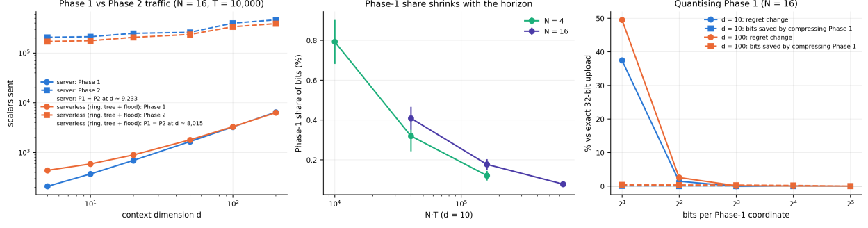
Figure 3: Empirical check of Proposition 15 (E24). Left: Phase-1 traffic grows linearly in d , Phase-2 traffic is far larger for every d \leq 200 , server and serverless. Middle: the Phase-1 share falls as NT grows, as O(d/(NT)^{1/3}) predicts. Right: quantising the Phase-1 upload saves at most 0.06–0.38% of all bits, while 2-bit rounding costs 37–50% regret.
