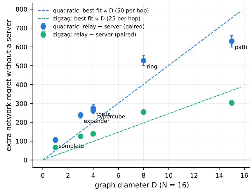
Cost of no server vs diameter ( T = 10,000 )
