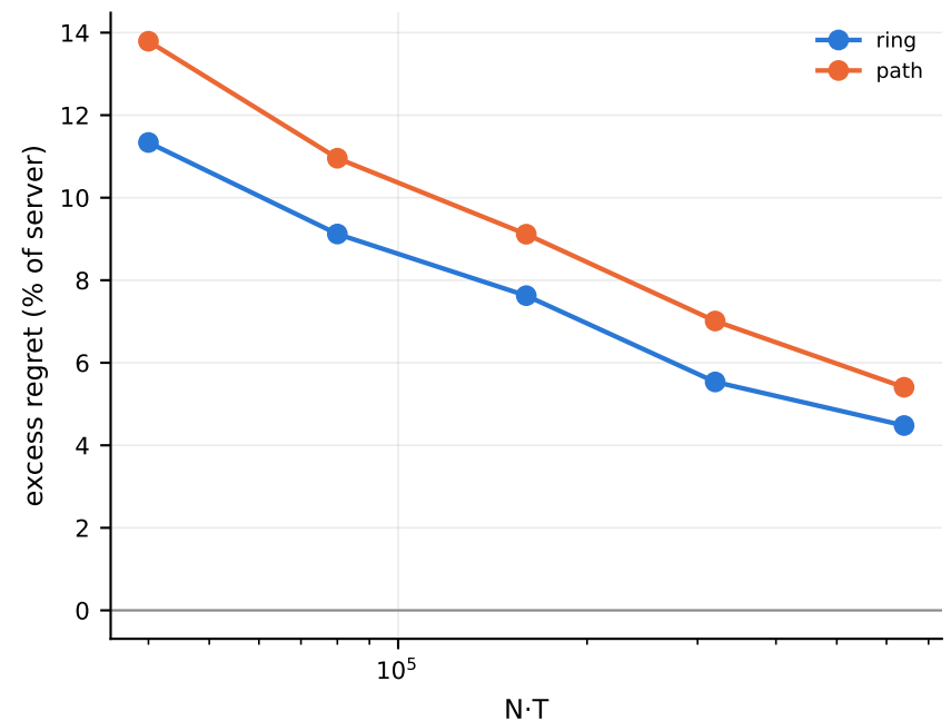
Relative cost of no server
