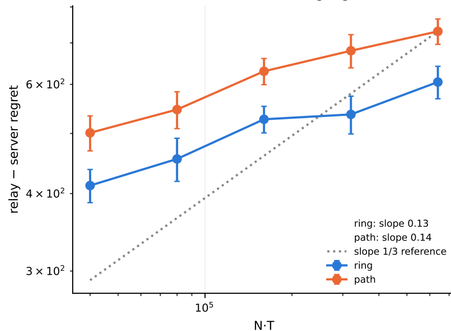
Excess vs horizon (log-log)
