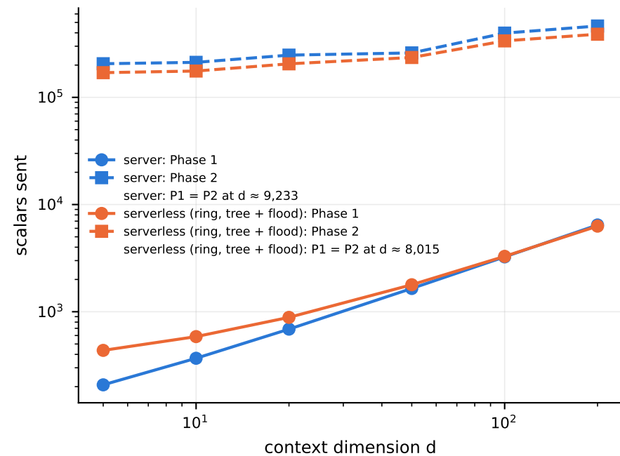
Phase 1 vs Phase 2 traffic (N = 16, T = 10,000)
