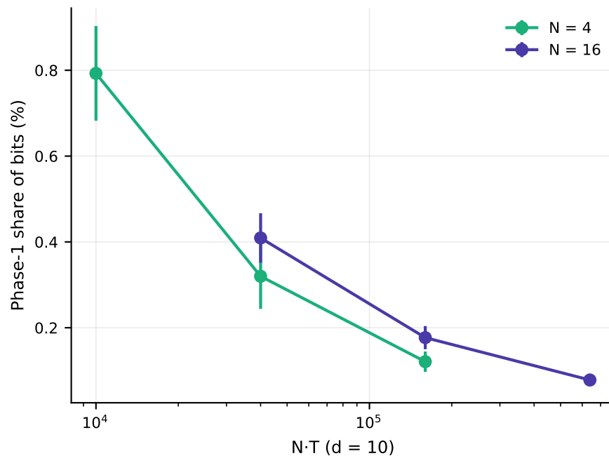
Phase-1 share shrinks with the horizon
