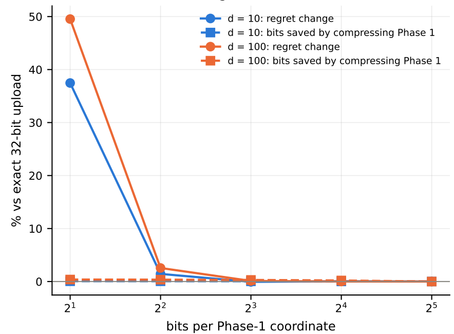
Quantising Phase 1 (N = 16)
