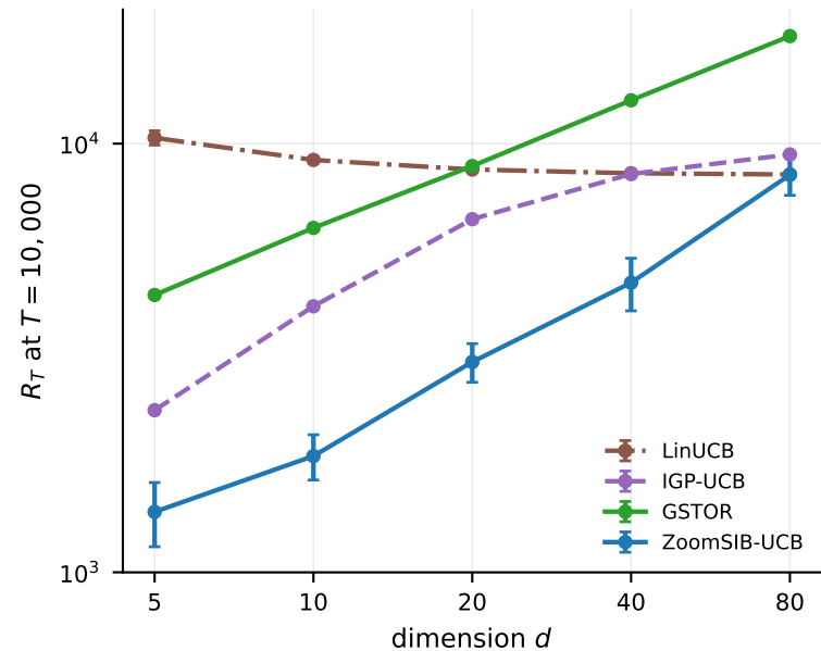
Final regret vs. dimension
