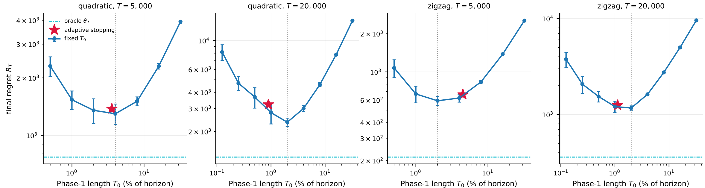
E4 · Phase-1 exploration trade-off (d=10, K=20, 15 trials, 95% CI)
