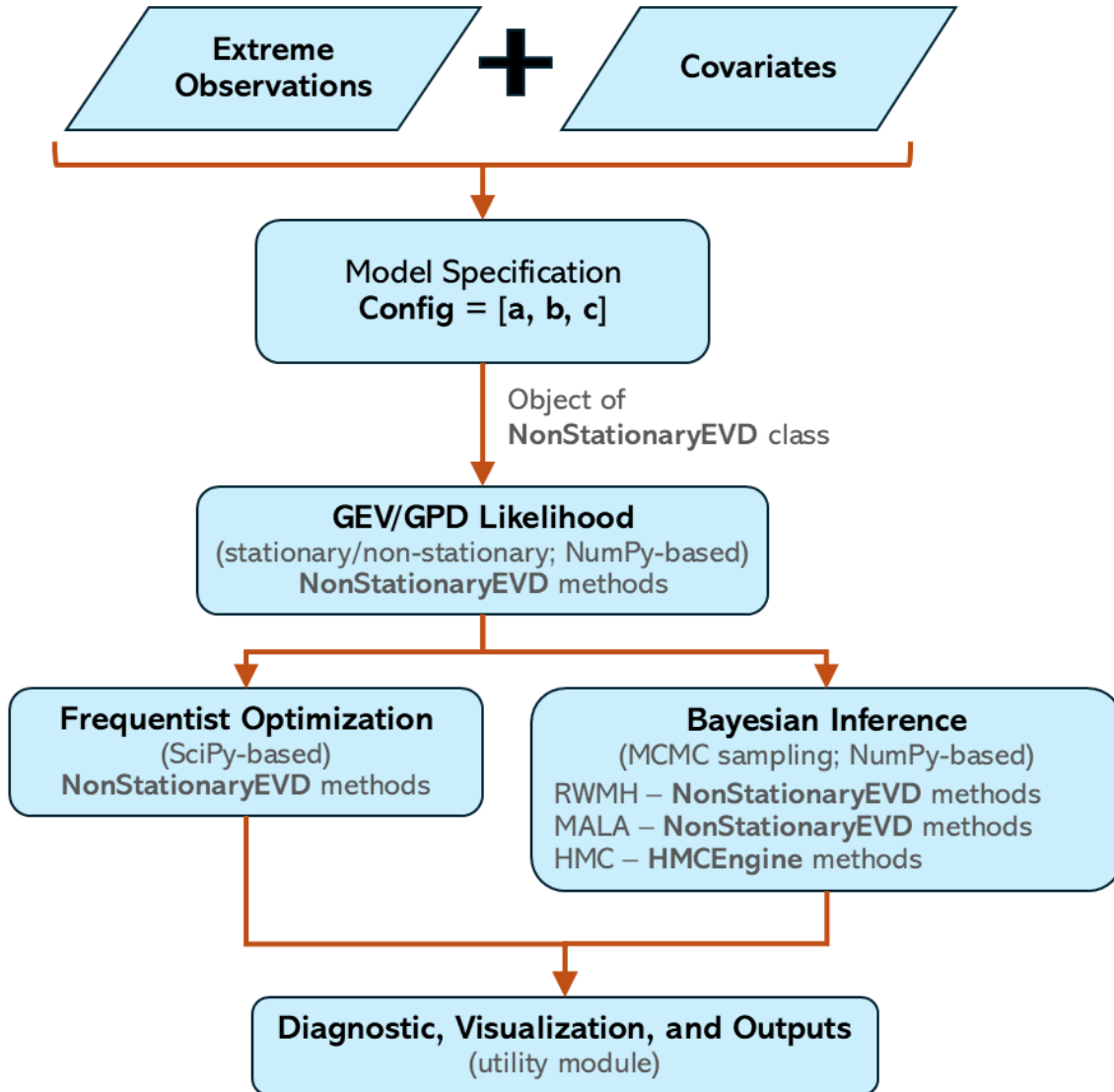
Figure 1: Workflow implemented in nsEVDx for specifying, fitting, and diagnosing stationary and non-stationary GEV and GPD models using frequentist optimization or Bayesian MCMC sampling
