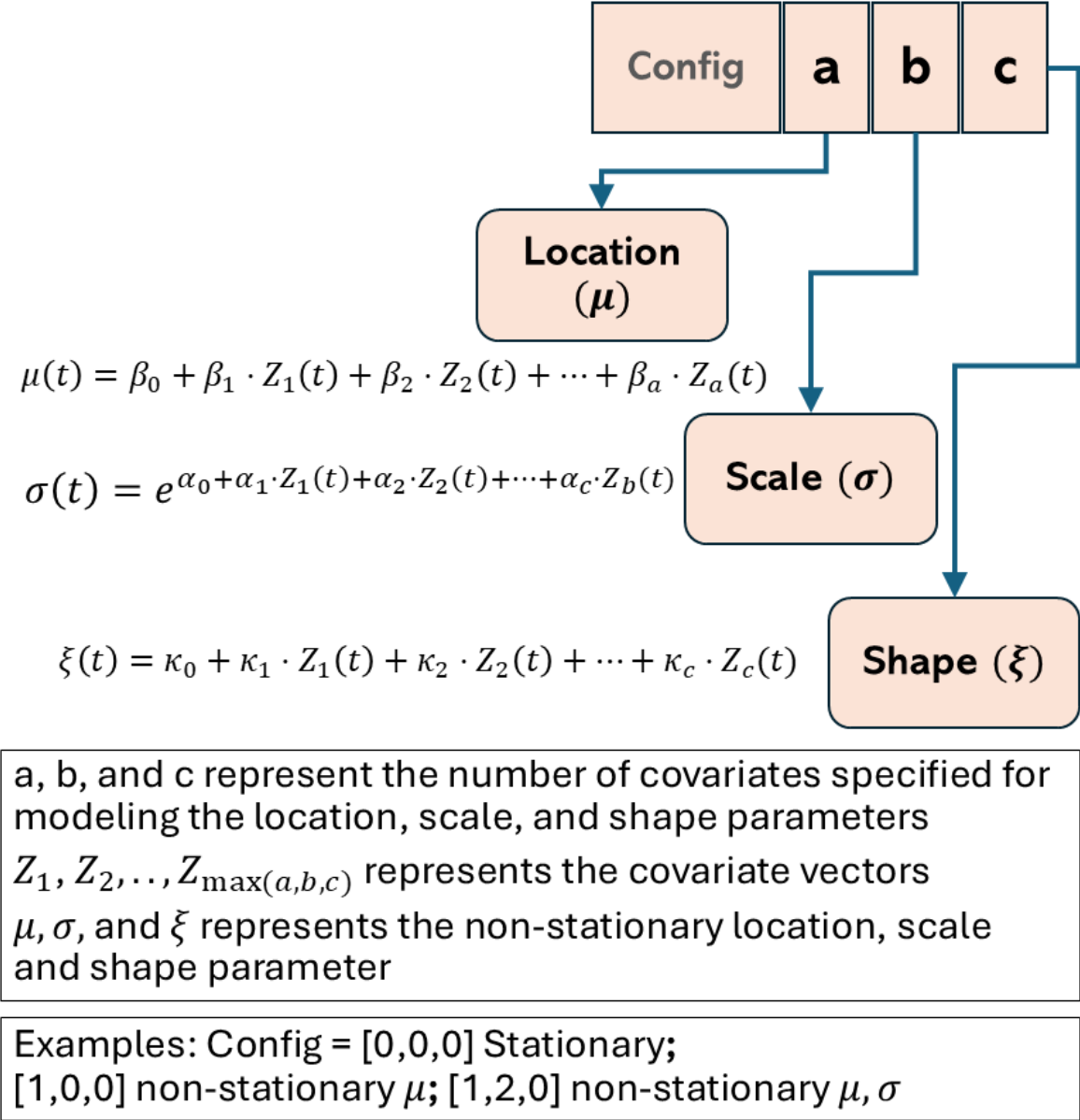
Figure 2: Configuration-vector framework used in nsEVDx for specifying stationary and non-stationary EVD models.
