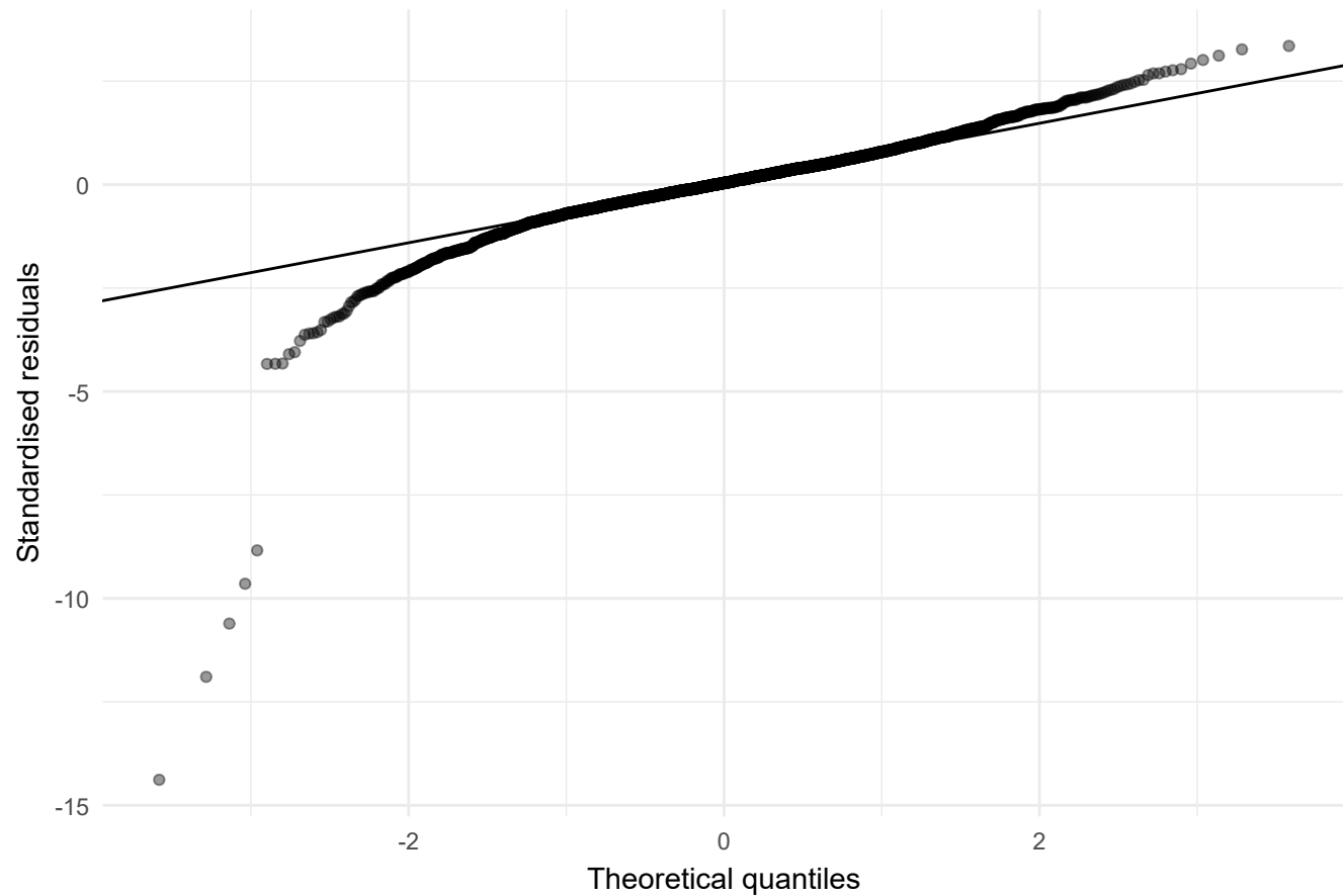
Normal Q-Q Plot of Standardised Residuals
