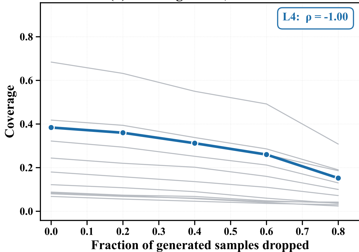
(b) Coverage: falls, as it must
