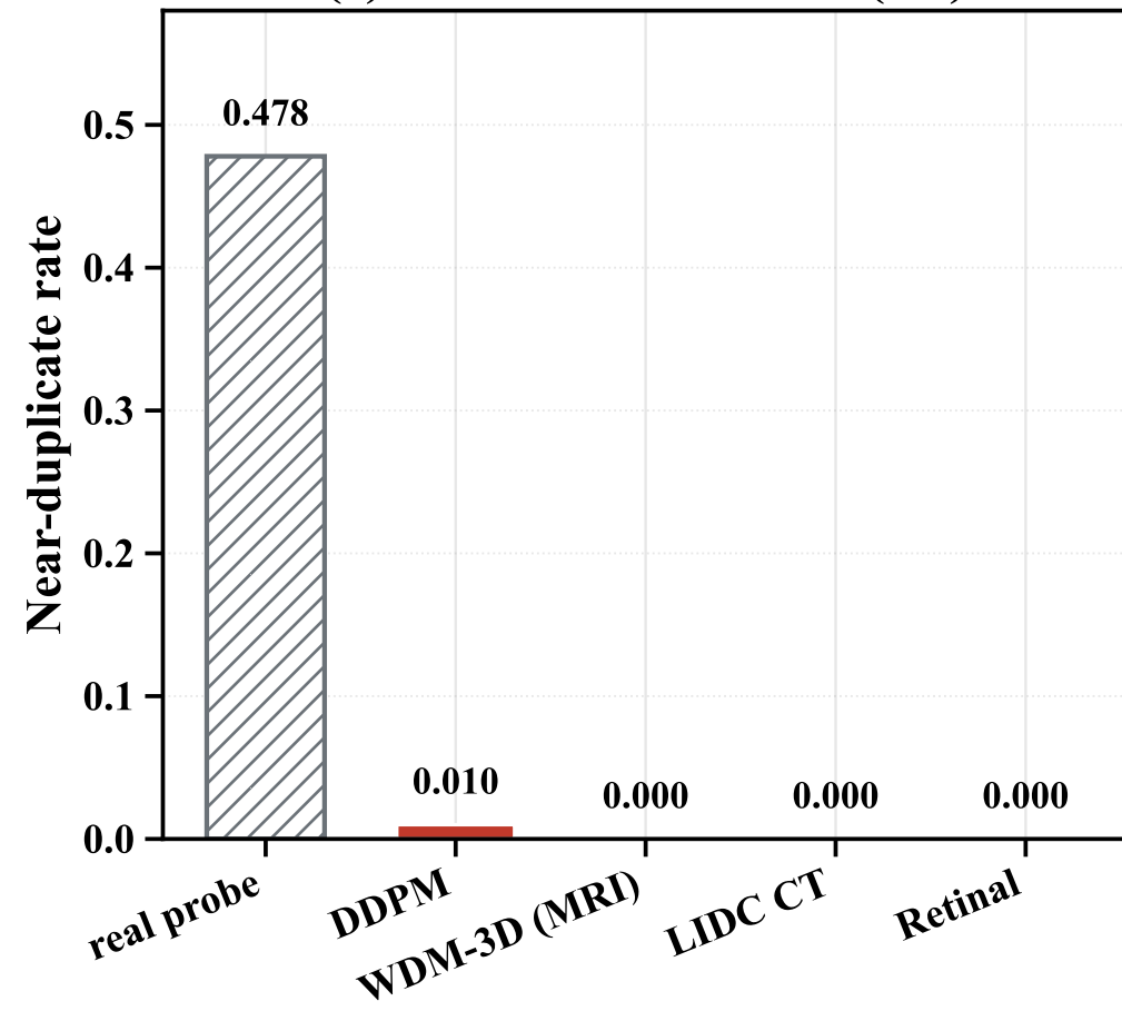
(c) Memorization rate (L9)
