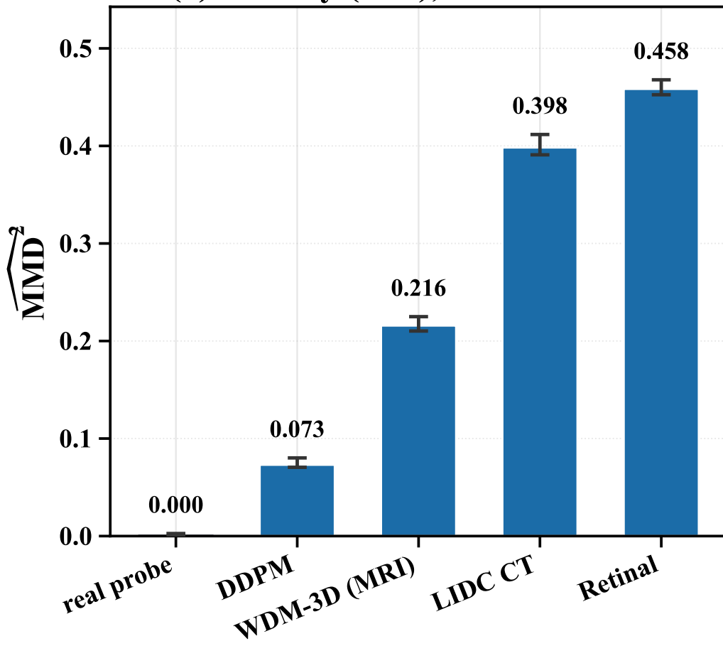
(a) Fidelity (L12), lower is better
