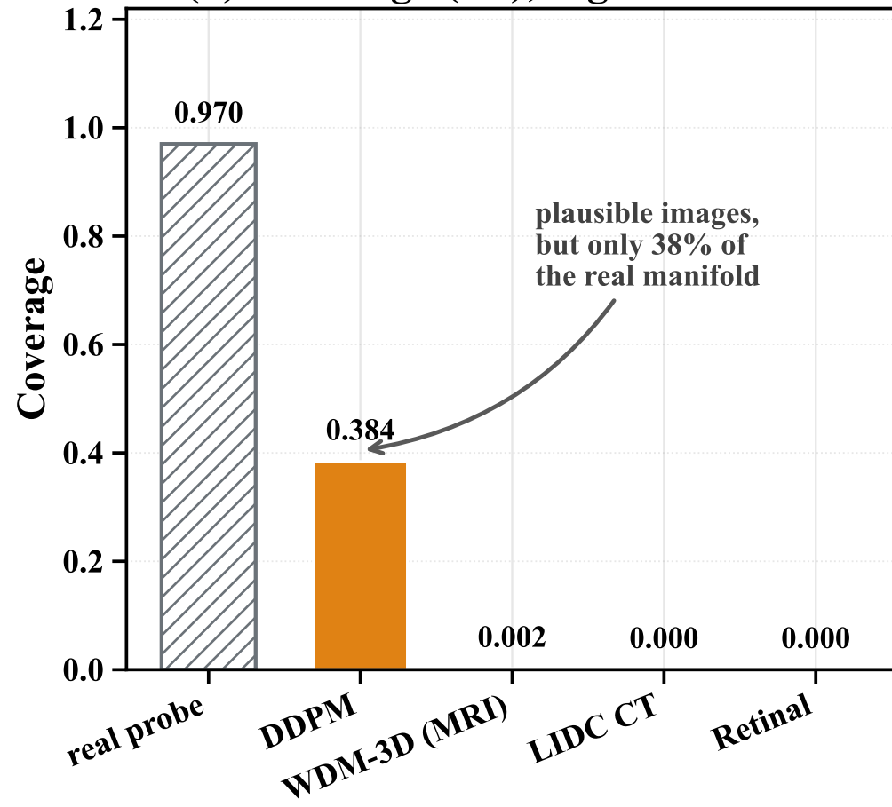
(b) Coverage (L4), higher is better
