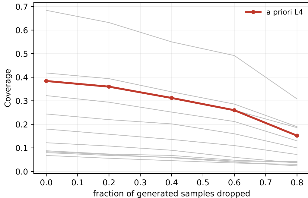
Coverage (Naeem et al.)
