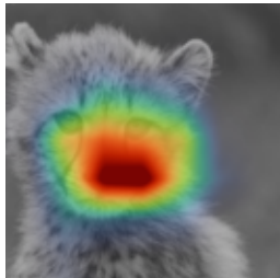
ResNet-50
