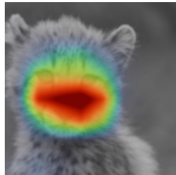
MobileViT
