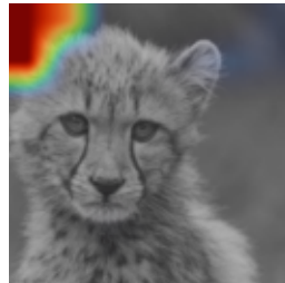
EffViT-B2
