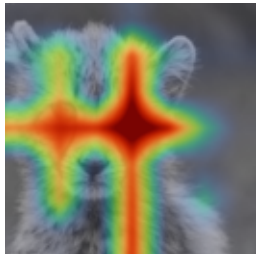
Swin-B
