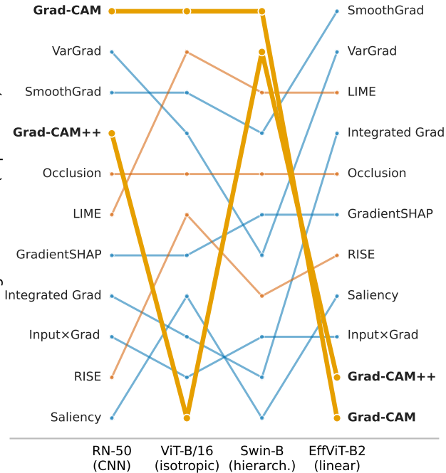
Pointing-Game rank (top = best)
