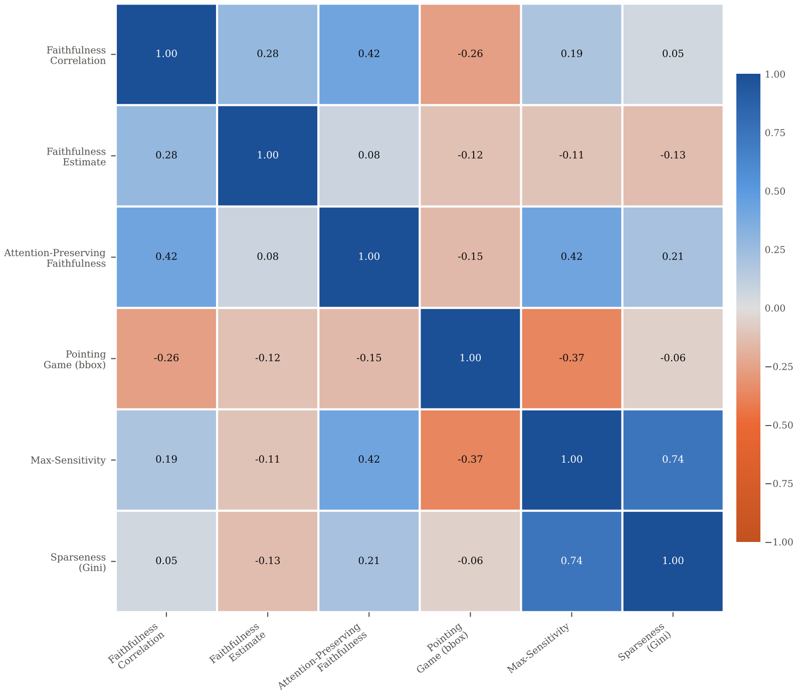
Spearman correlation between evaluation dimensions (over 117 model x method cells)
