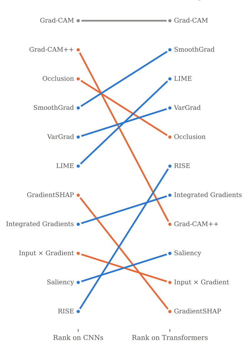
Rank transfer — 10/11 methods change rank
