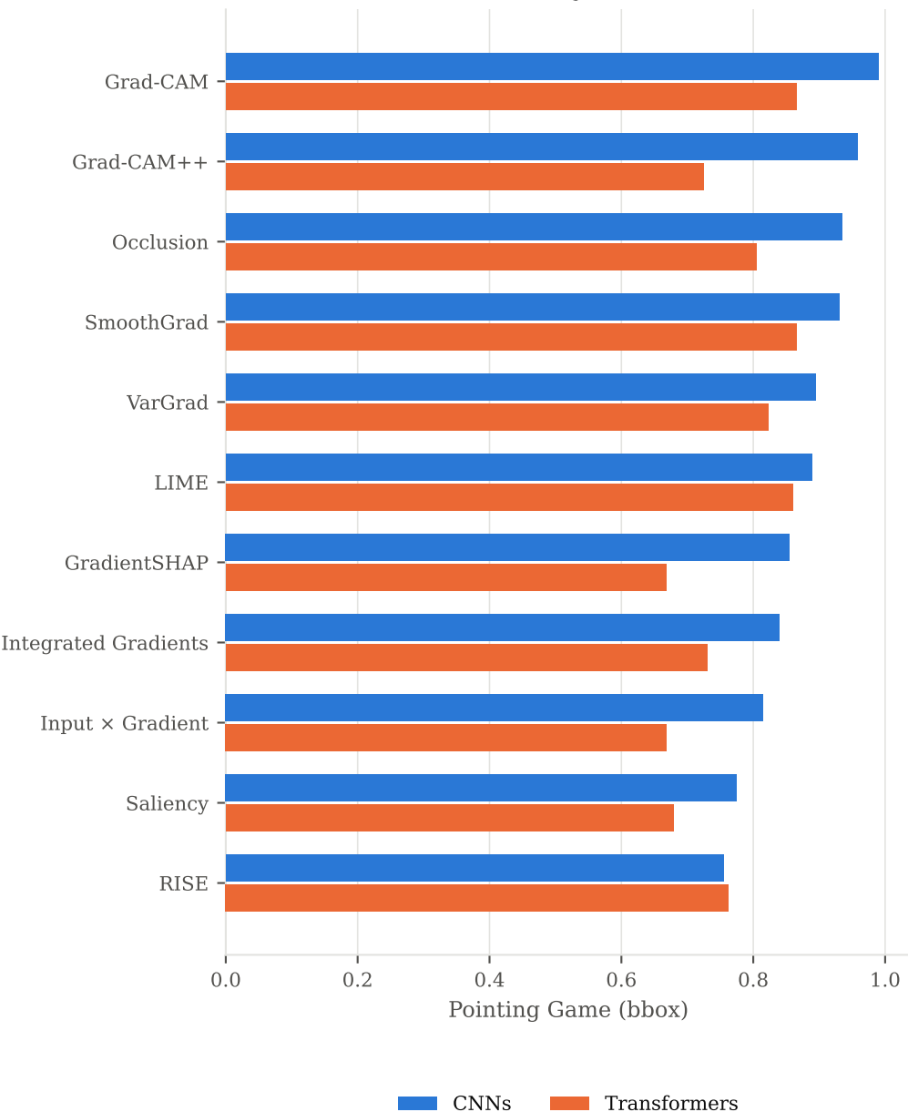
Localisation score by architecture class
