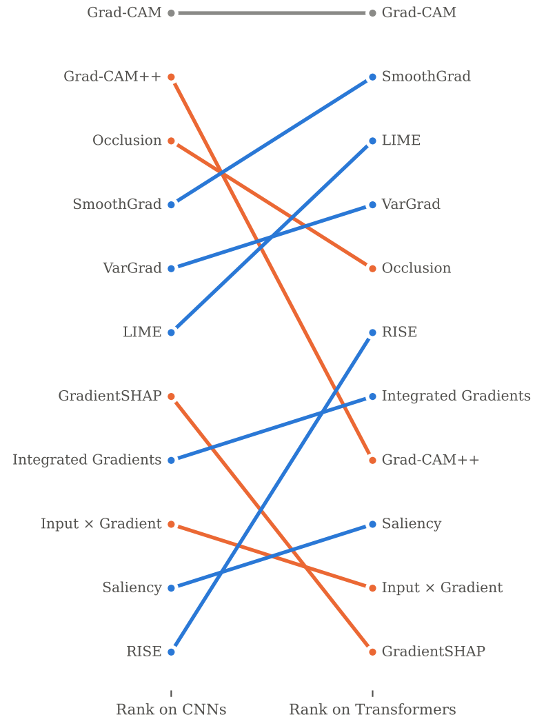
Rank transfer — 10/11 methods change rank
