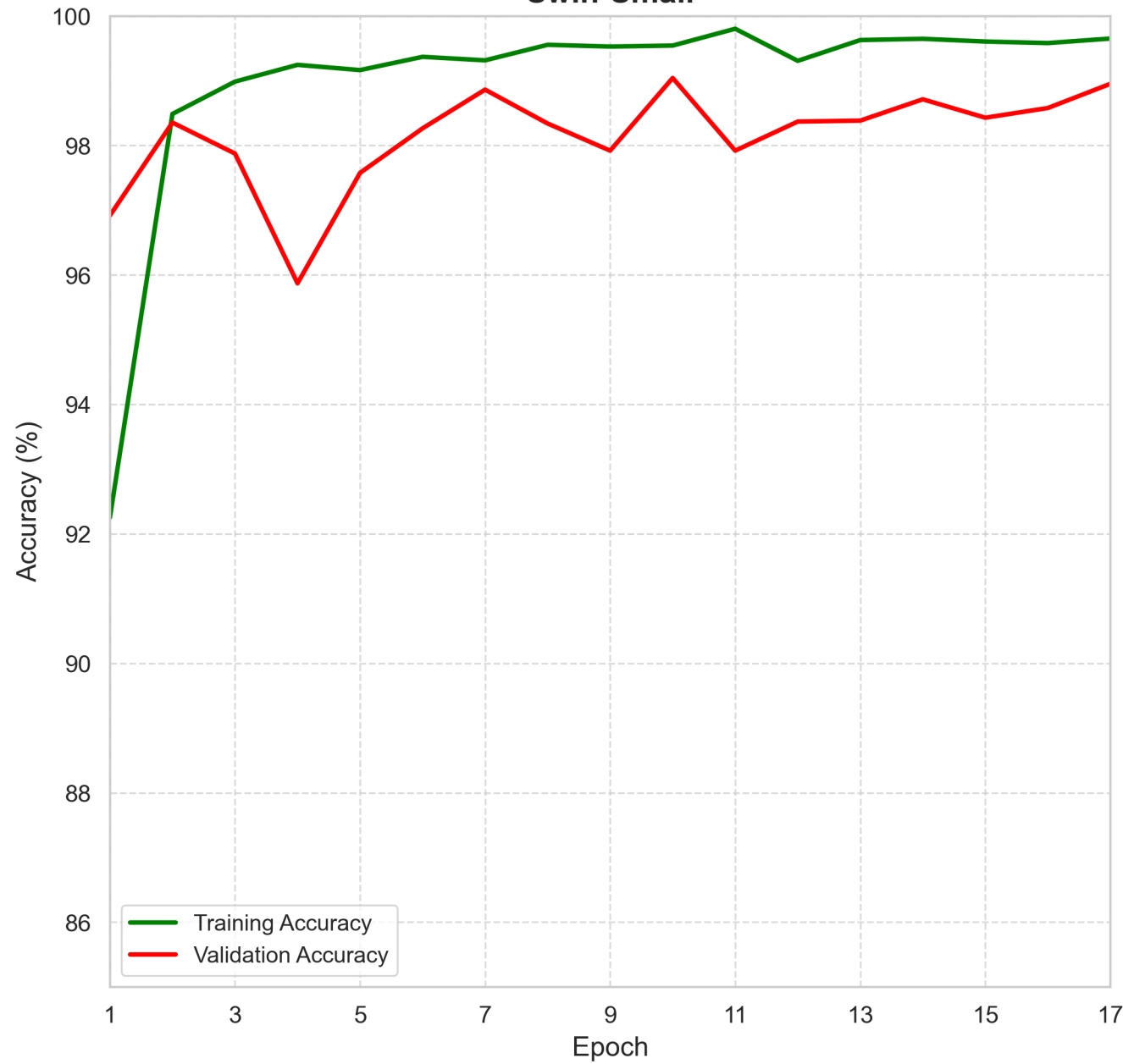
Swin-Small
