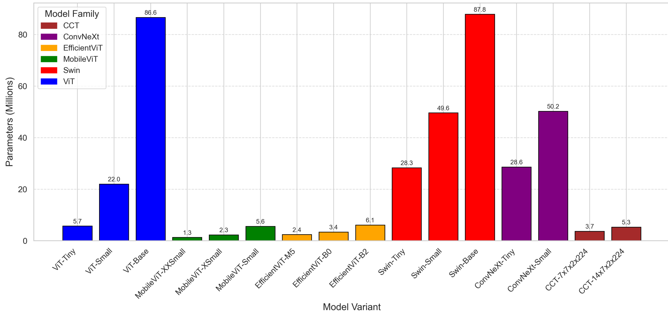
Parameter Counts for ViT-RoT Model Variants
