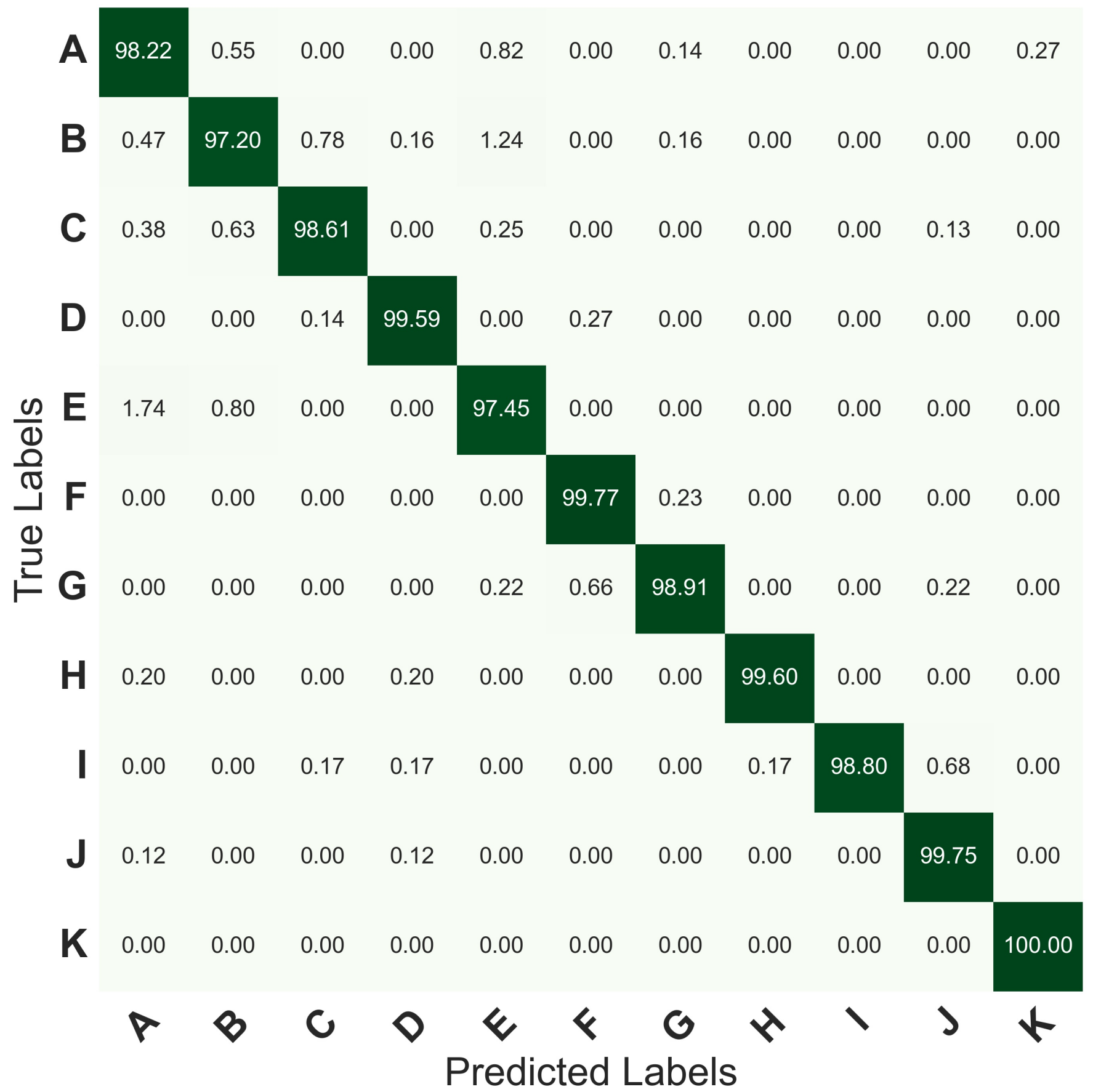
Convnext Small
