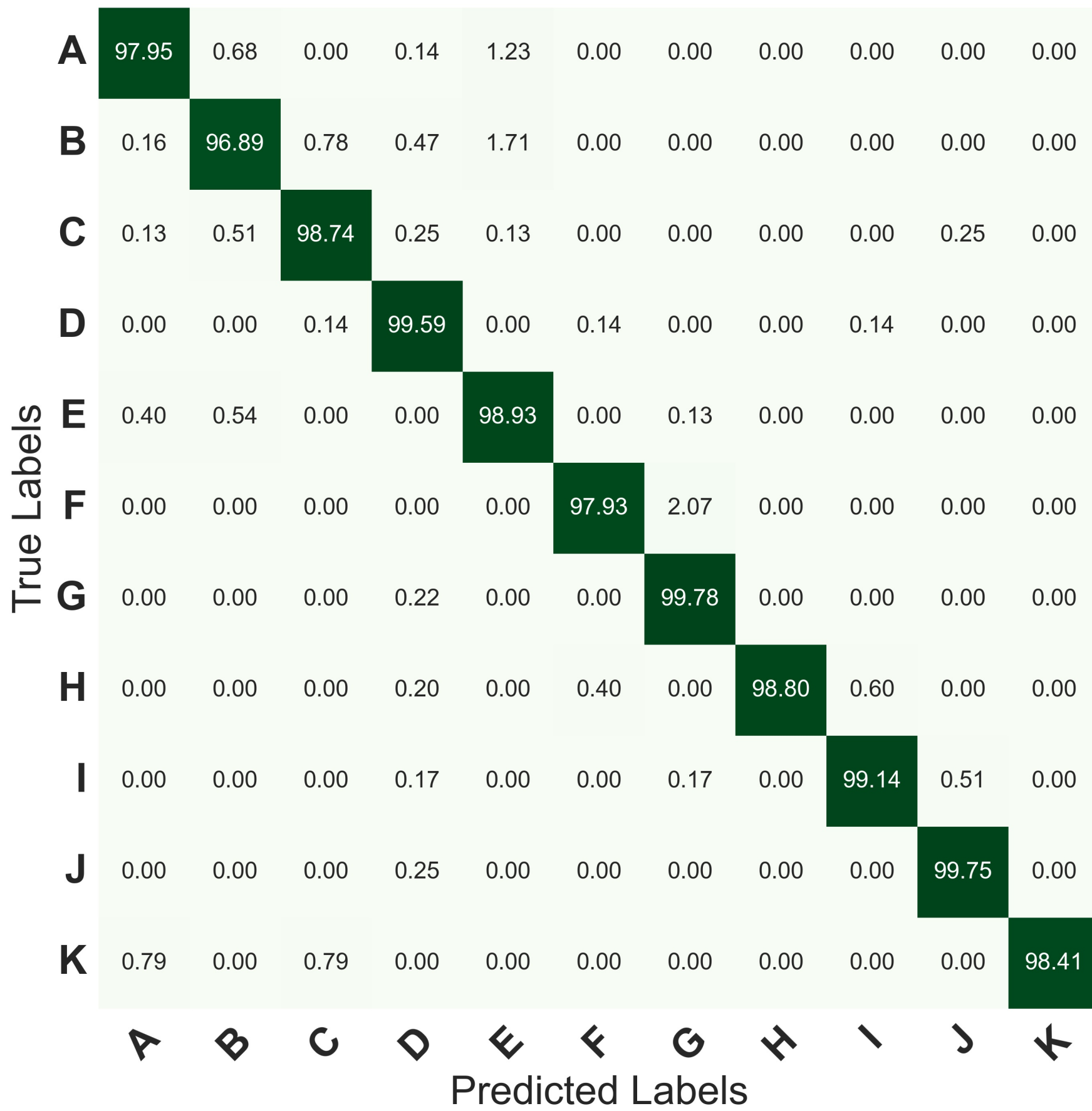
Swin Small
