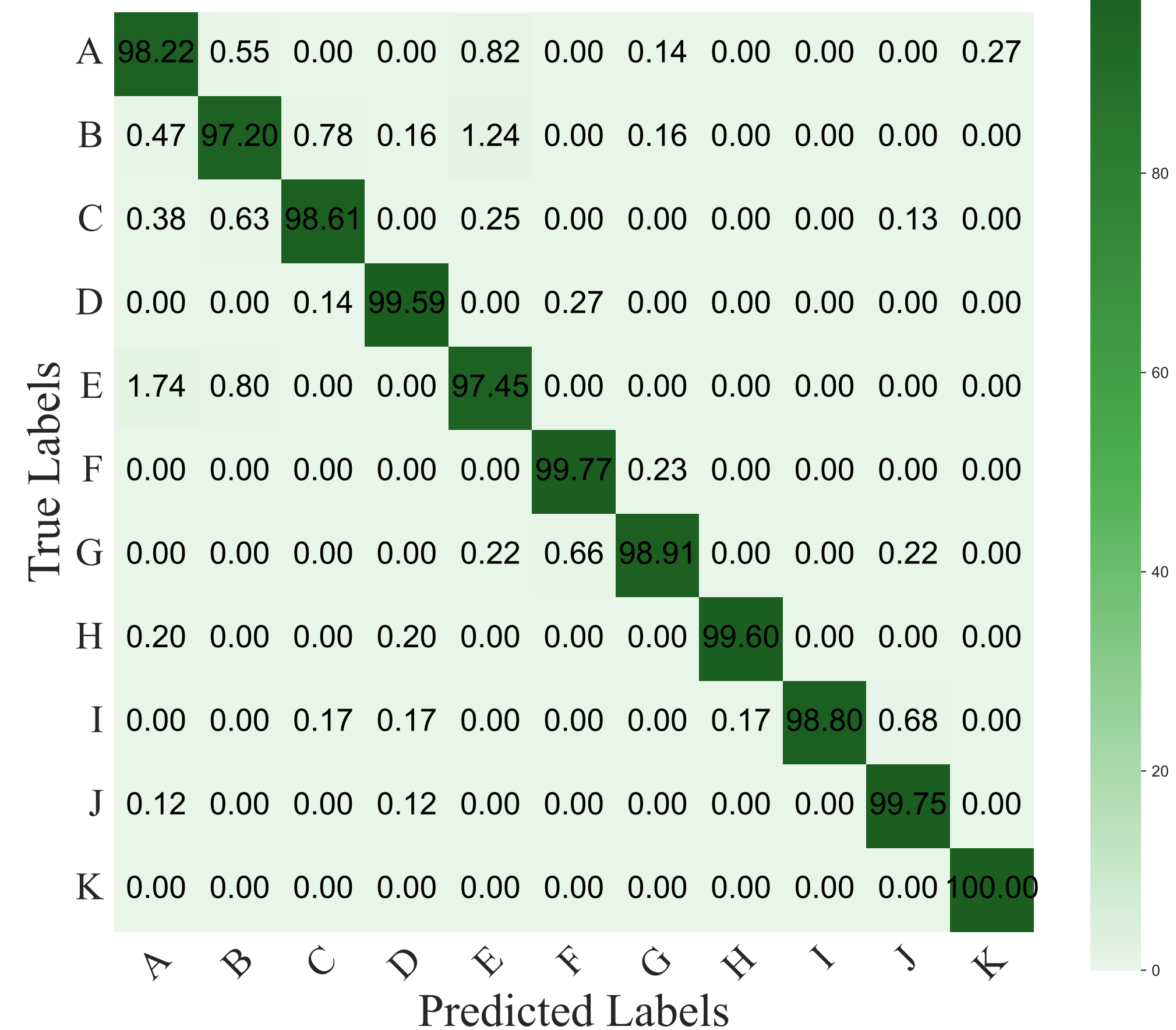
ConvNext Small
