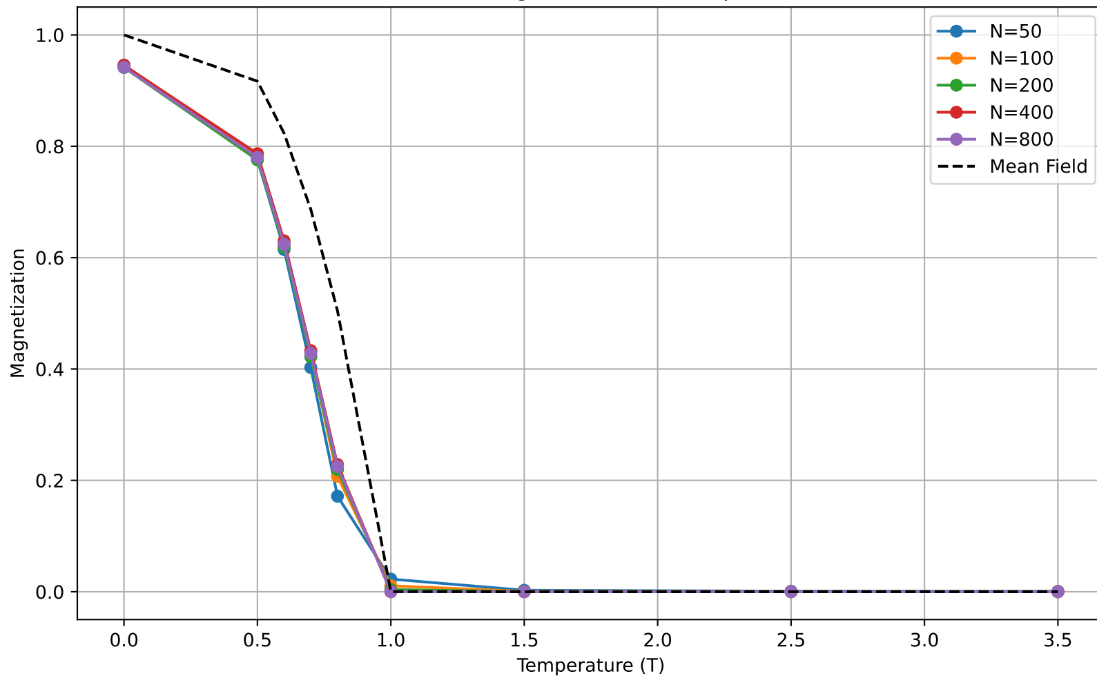
Finite Size Magnetization vs Temperature
