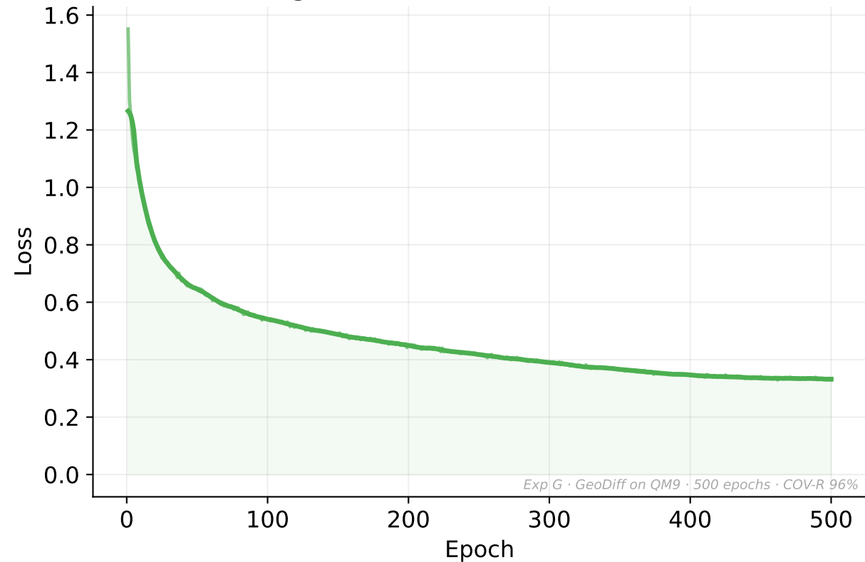
Score-Matching MSE Loss (Coordinate Noise Prediction)
