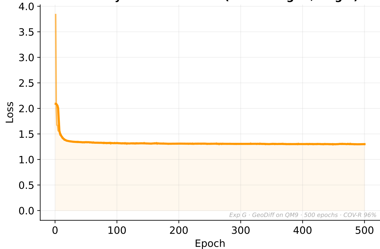
Geometry Constraint Loss (Bond Length / Angle)
