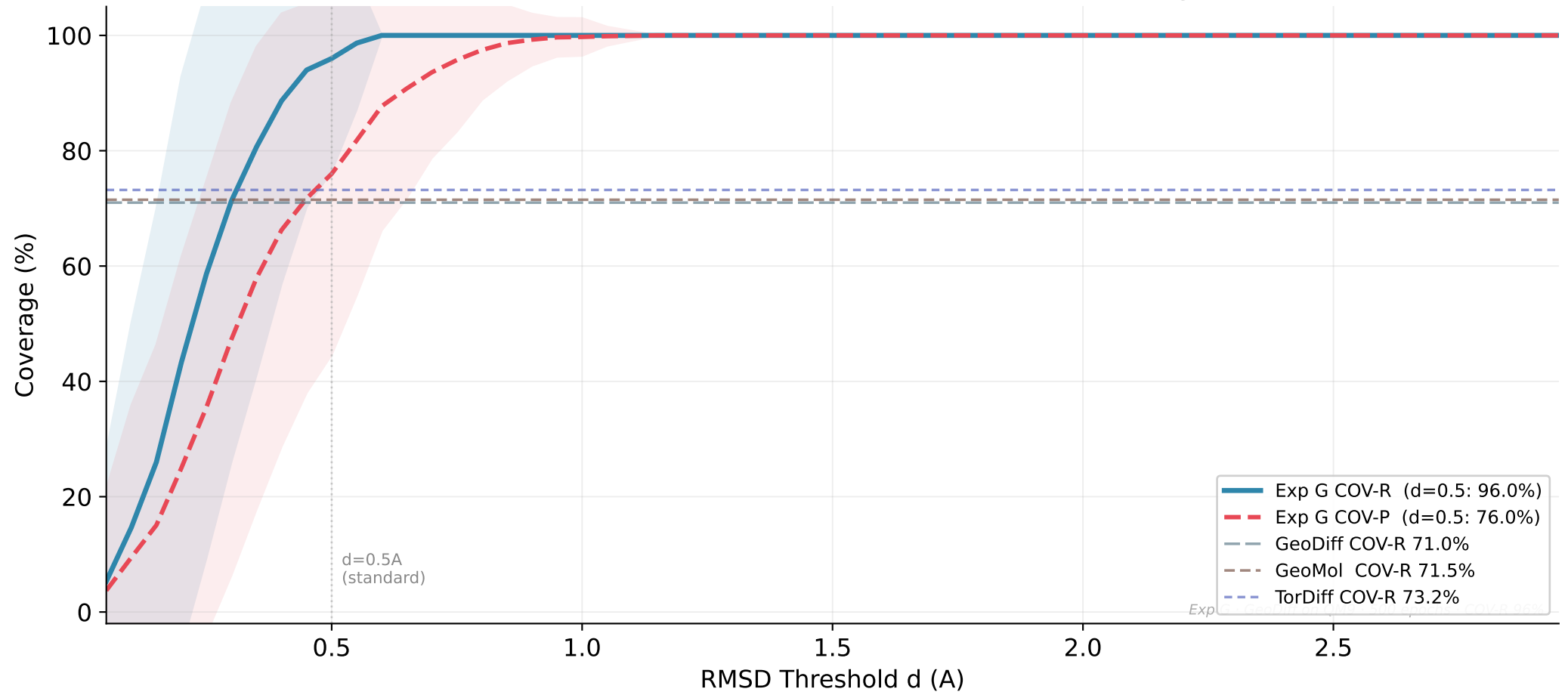
Exp G (QM9) — Coverage vs RMSD Threshold [COV-R & COV-P] (swept 0.05-3.0 Å; shaded = +/-1 std across molecules; n=10 generated/mol)
