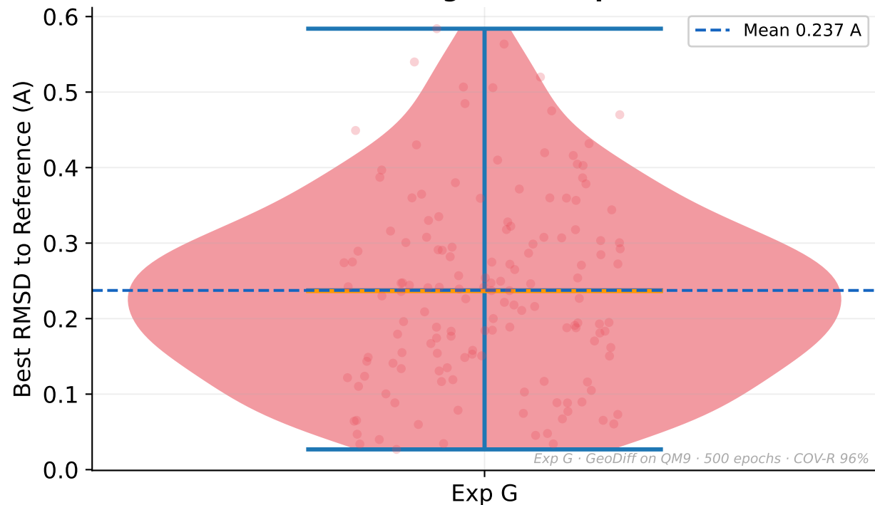
Best-Generated RMSD Distribution (min over 10 generated per mol)
