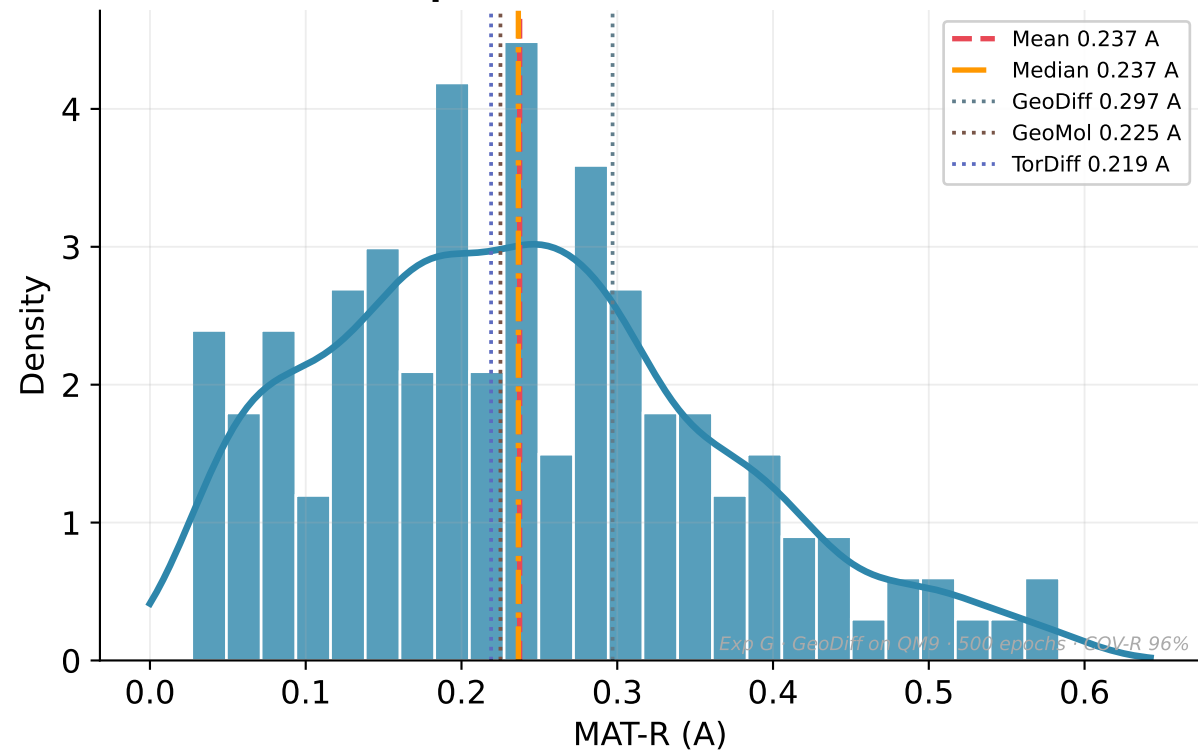
MAT-R Distribution (competitive with TorDiff SOTA!)
