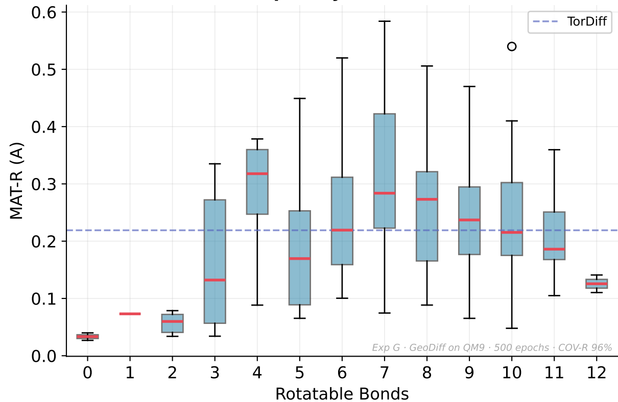
MAT-R Boxplot by Rotatable Bonds
