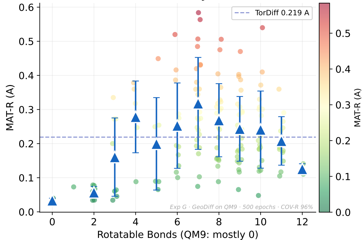
MAT-R vs Flexibility (scatter)
