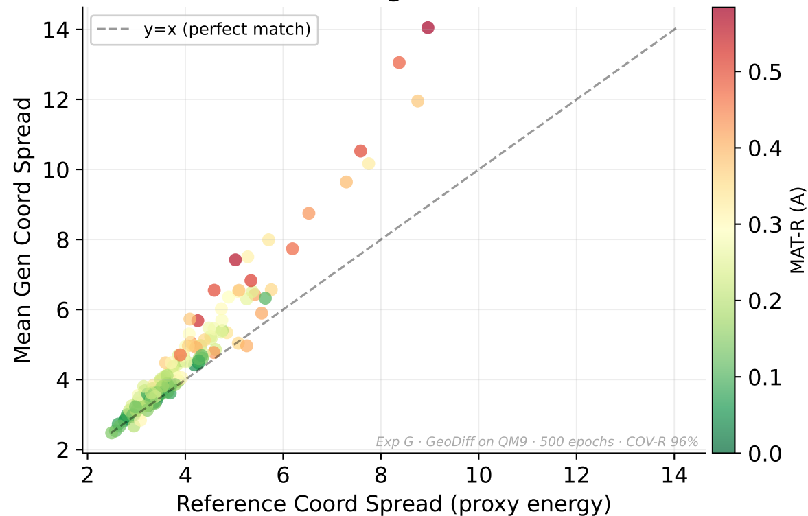
Generated vs Reference Coordinate Scale (color=MAT-R; near diagonal = well-calibrated)
