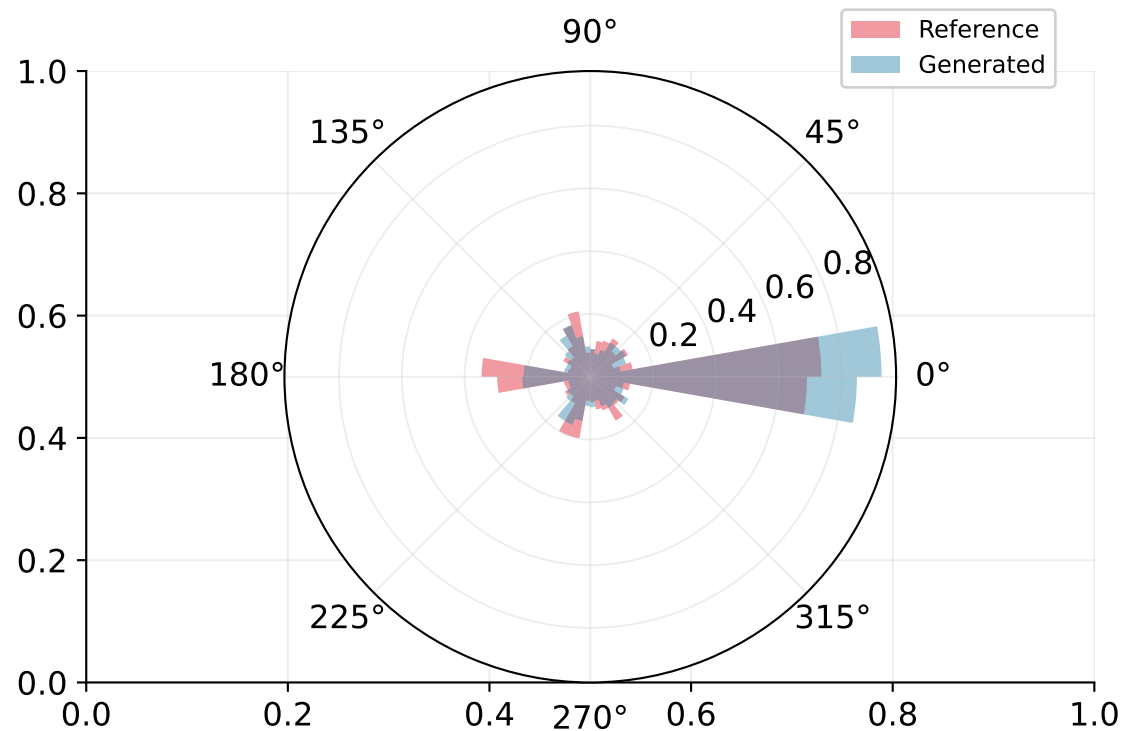
Torsion Rose Diagram
