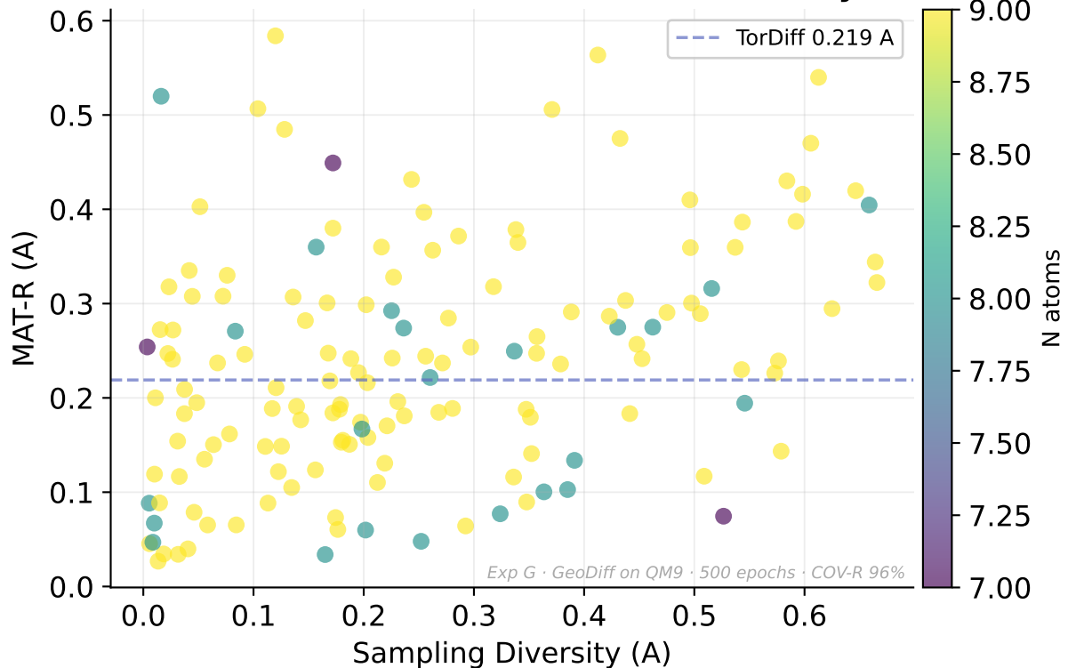
Quality-Diversity Trade-off (QM9: lower MAT-R + moderate diversity)
