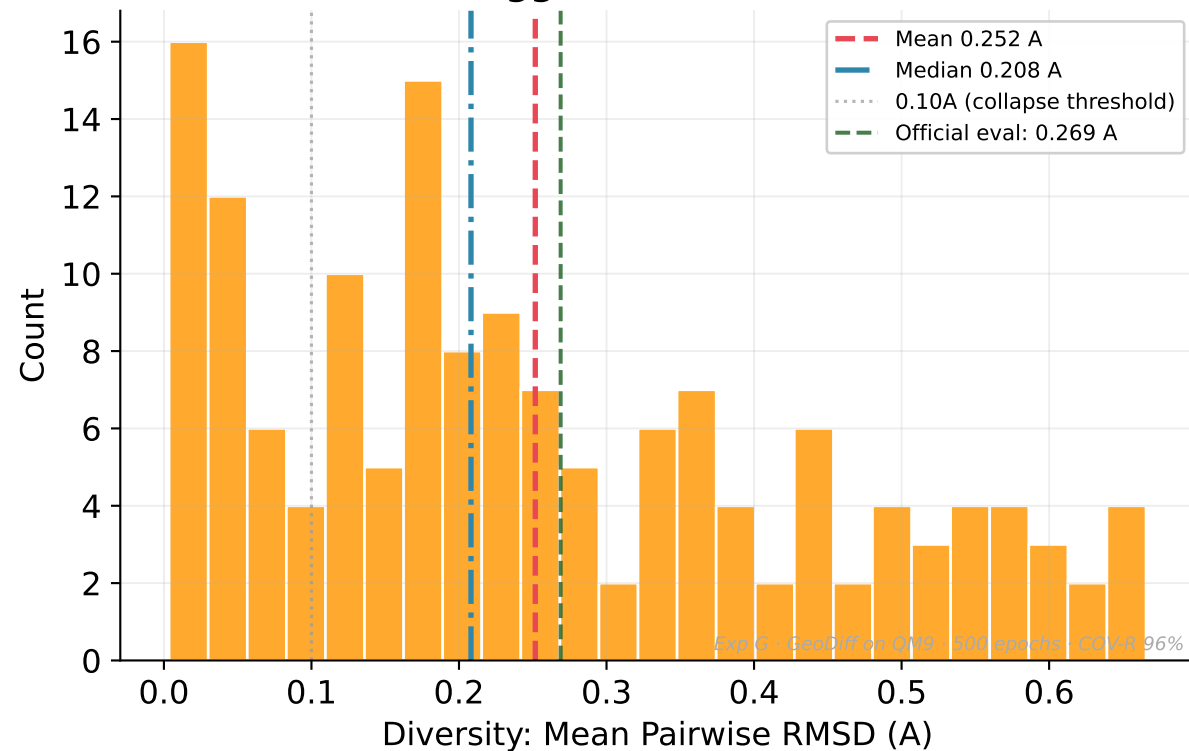
Conformer Sampling Diversity (official logged eval: 0.269 A mean)
