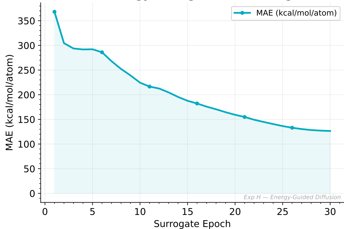
Phase 1: Energy Surrogate Pre-training (MAE)
