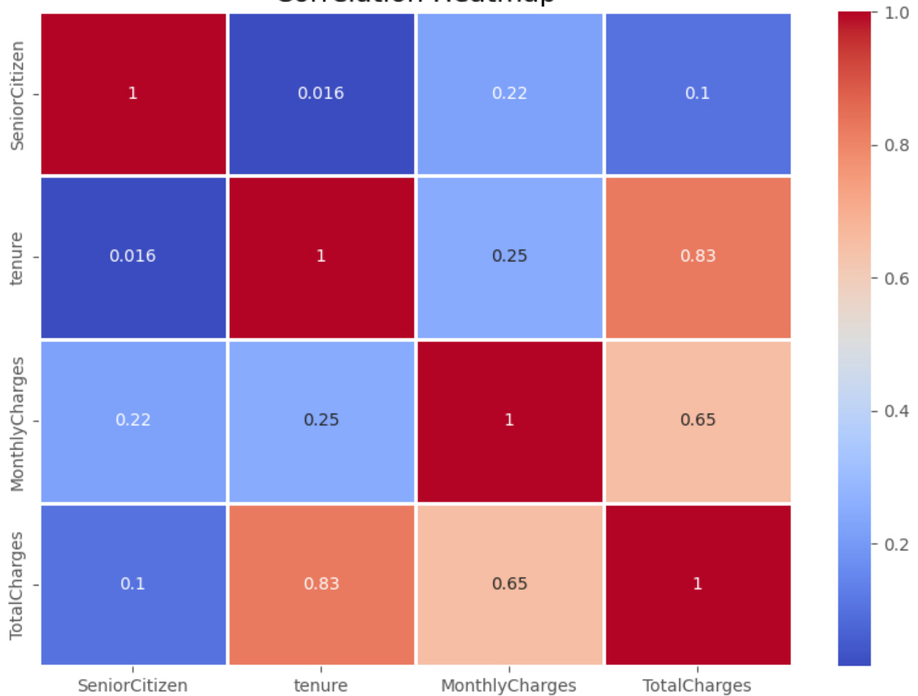
Correlation Heatmap
