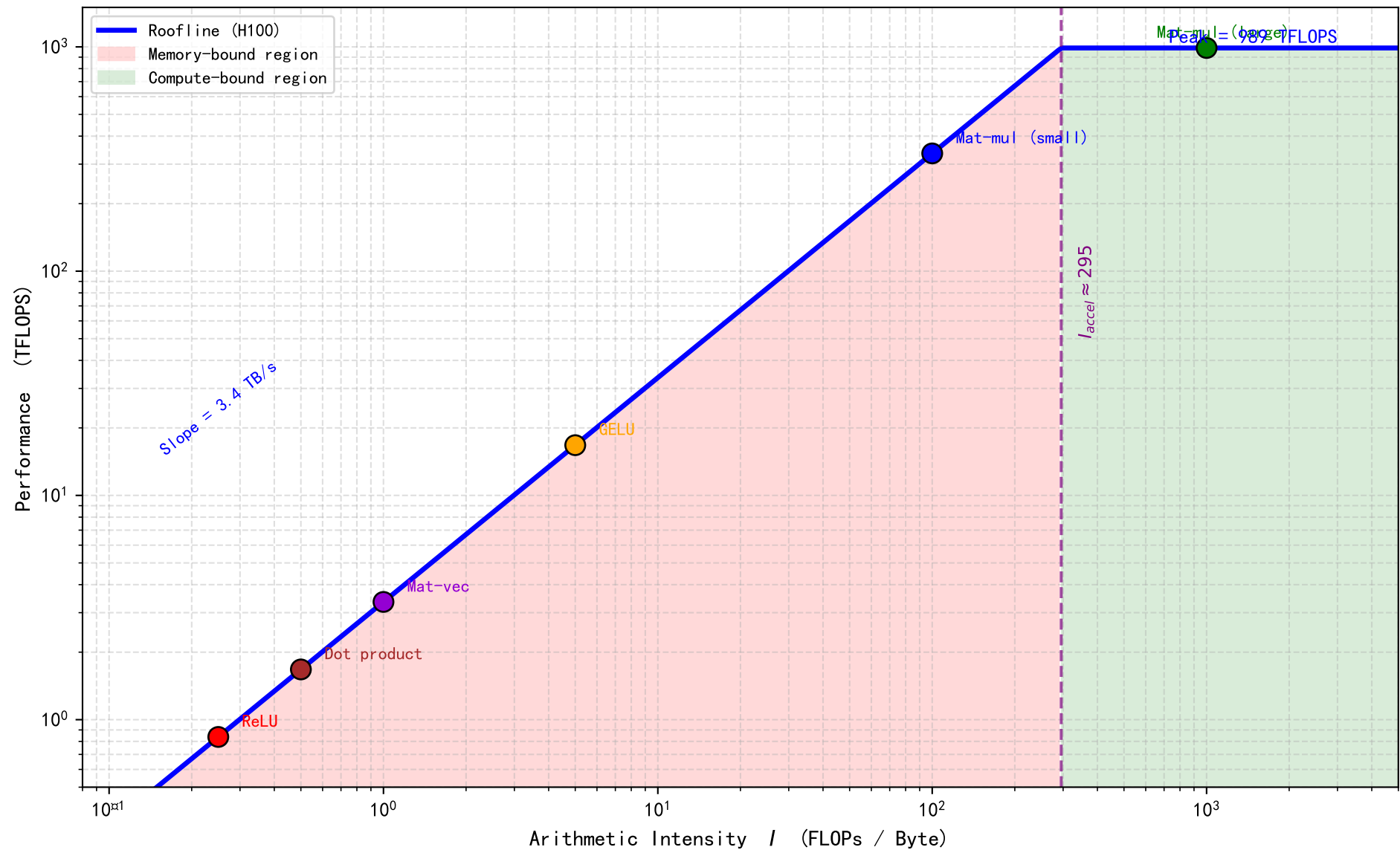
Roofline Model (NVIDIA H100, BF16 Dense)
