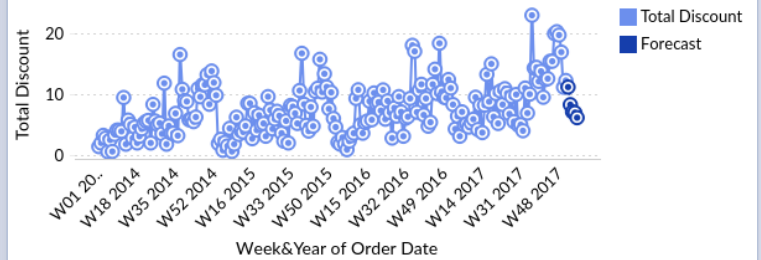
Discount across Weeks with Forecast
