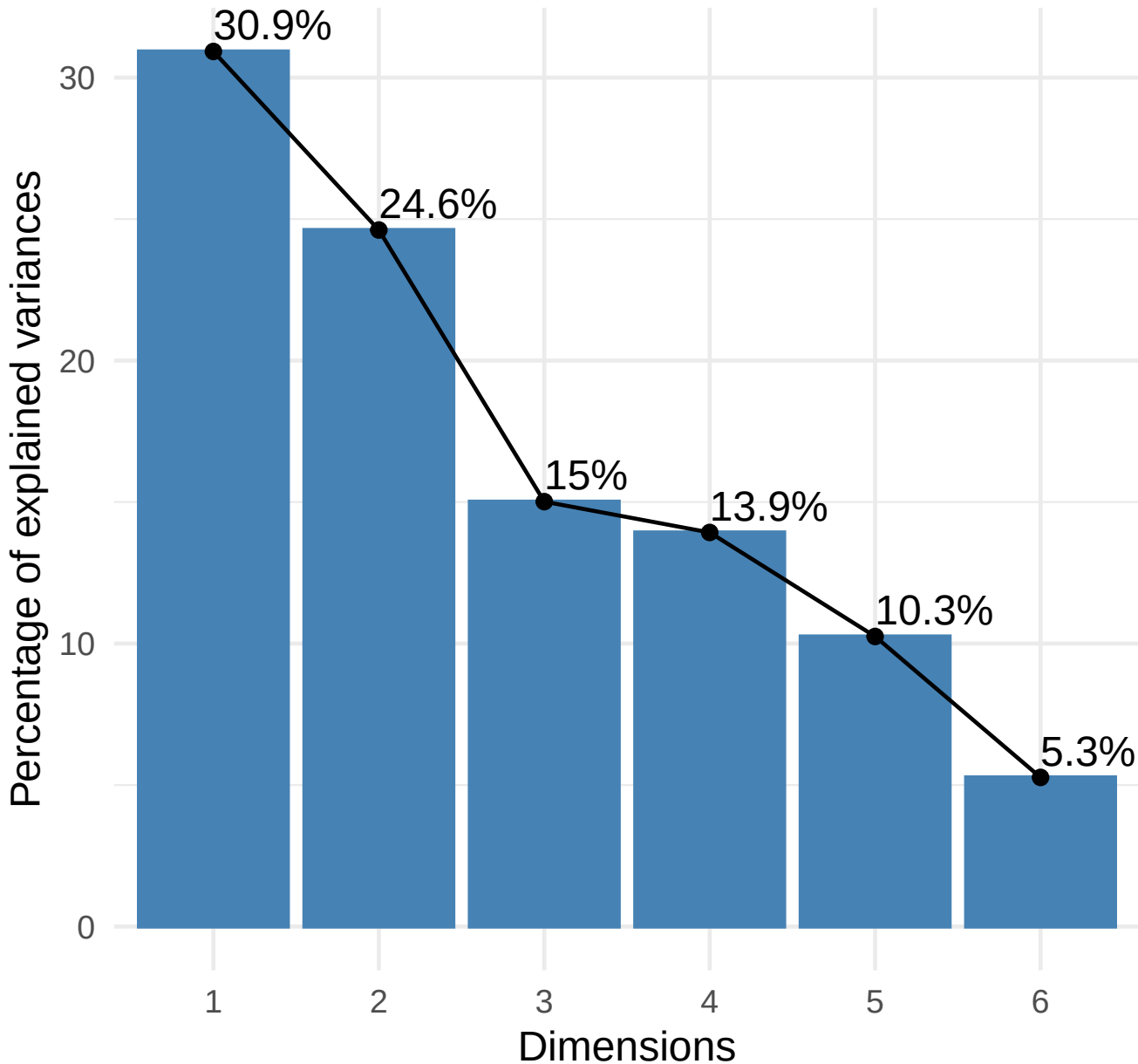
Scree Plot: Variance Explained by Each PC
