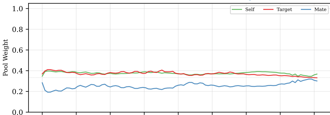
P0 (Striker) — Learned Attention Pooling
