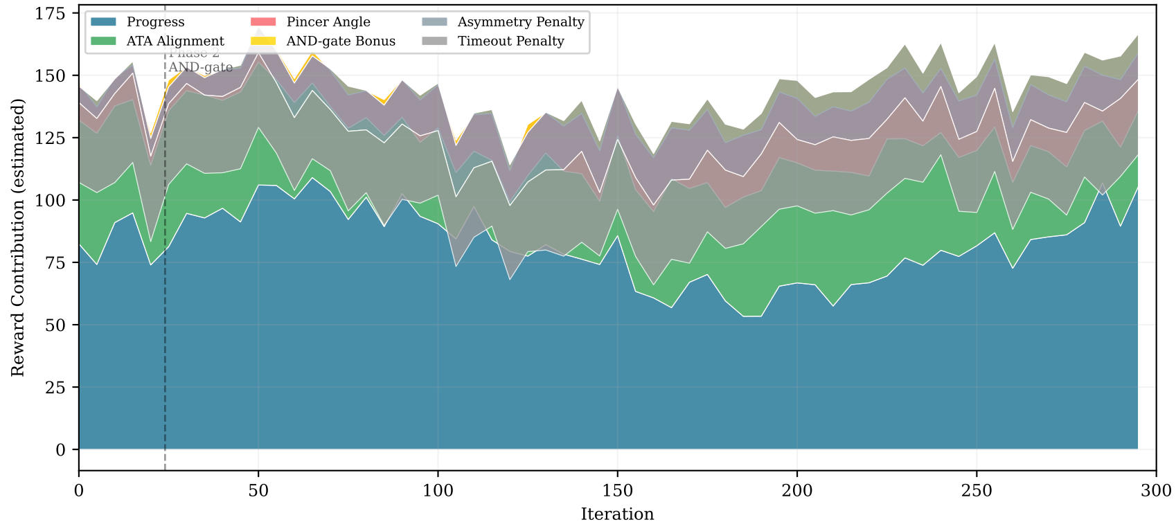
Reward Component Breakdown — Curriculum Learning Effect (Exp 3v3 Dynamic Annealing Structure)
