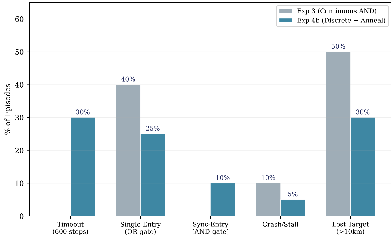
Termination Reason Distribution — Discrete + Annealing vs Continuous AND
