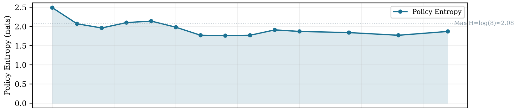
Policy Entropy — Healthy Convergence (2.49 \rightarrow 1.87)
