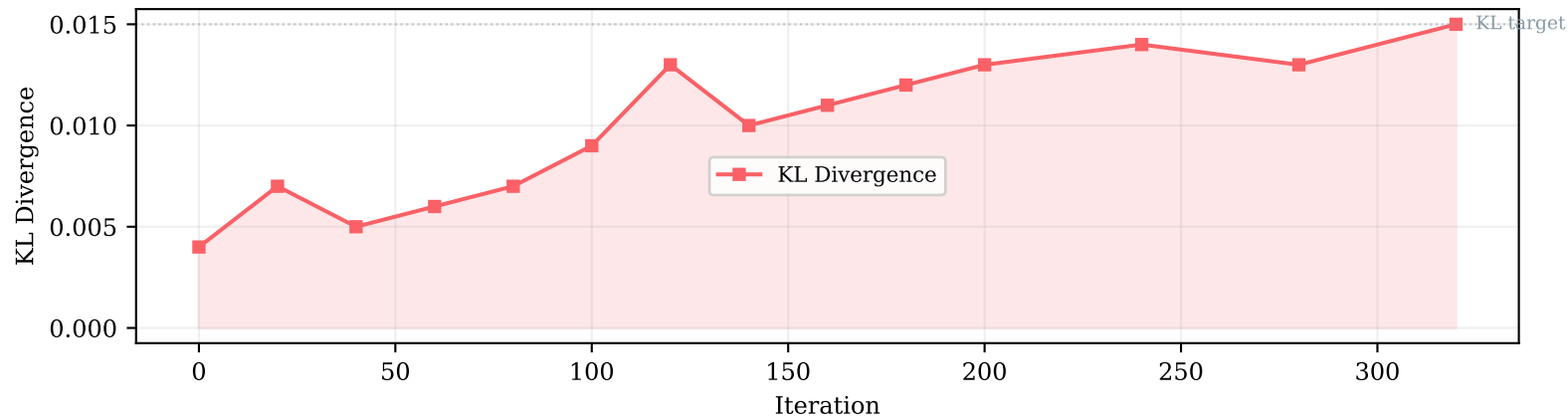
KL Divergence — Controlled Updates (0.004 \rightarrow 0.015)
