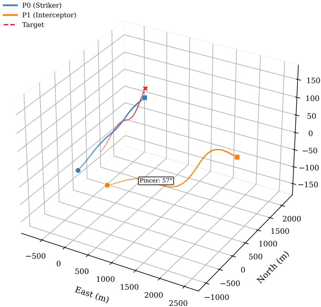
3D Formation Pursuit Trajectory — Parameter-Shared MAPPO (CTDE) d0_min=200m, d1_min=1307m, Pincer max=57°
