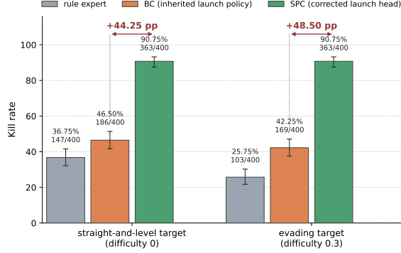
Figure 3: Difficulty robustness. Kill rate by policy at d=0 and d=0.3 (primary protocol, Wilson 95% intervals). The paired SPC–BC gap widens from +44.25 to +48.50 pp; discordant counts are 177 and 194, all favouring the correction.
