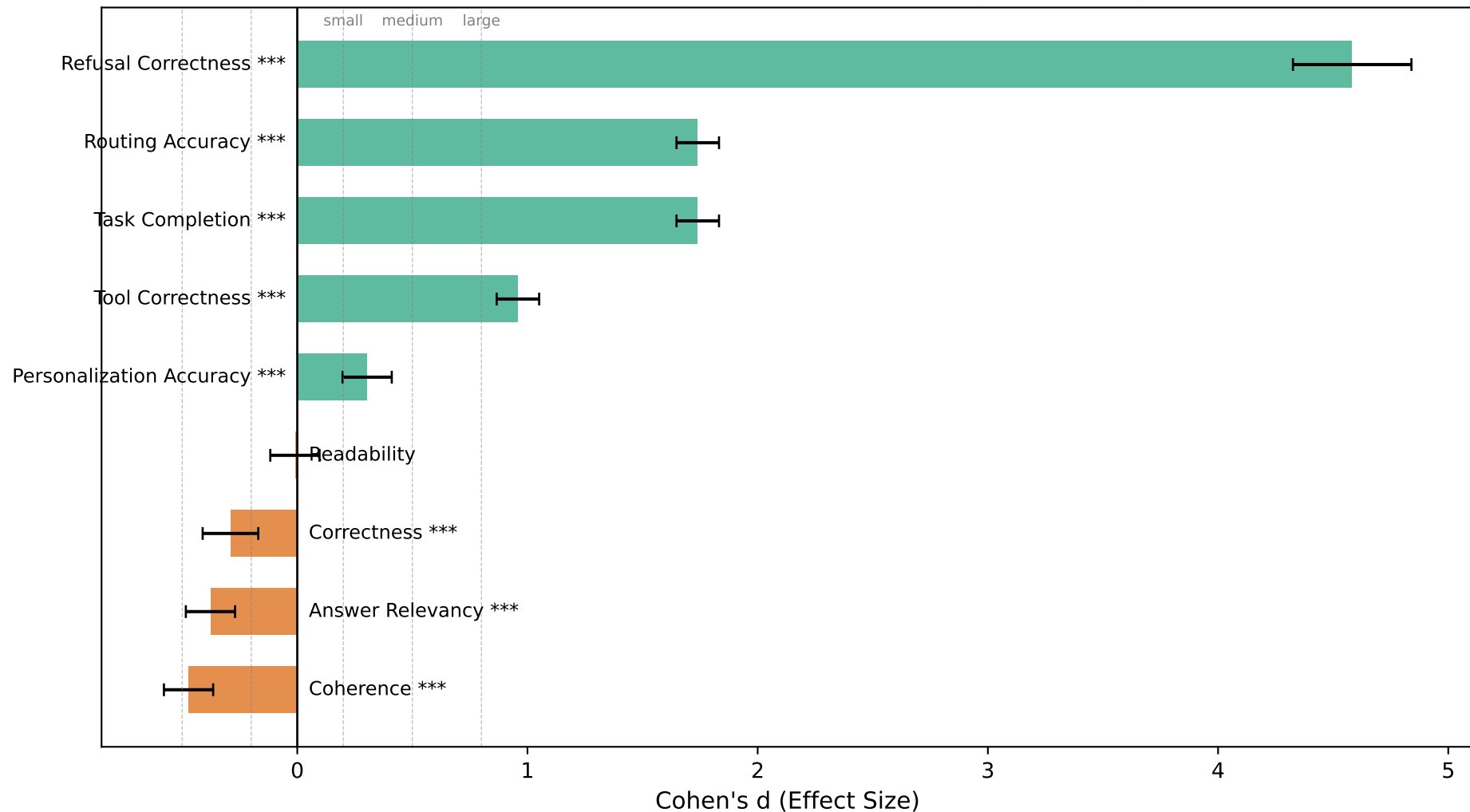
PRISM vs Baseline: Per-Metric Effect Size (green = PRISM better, orange = baseline better; * p < 0.05 , *** p < 0.001 )
