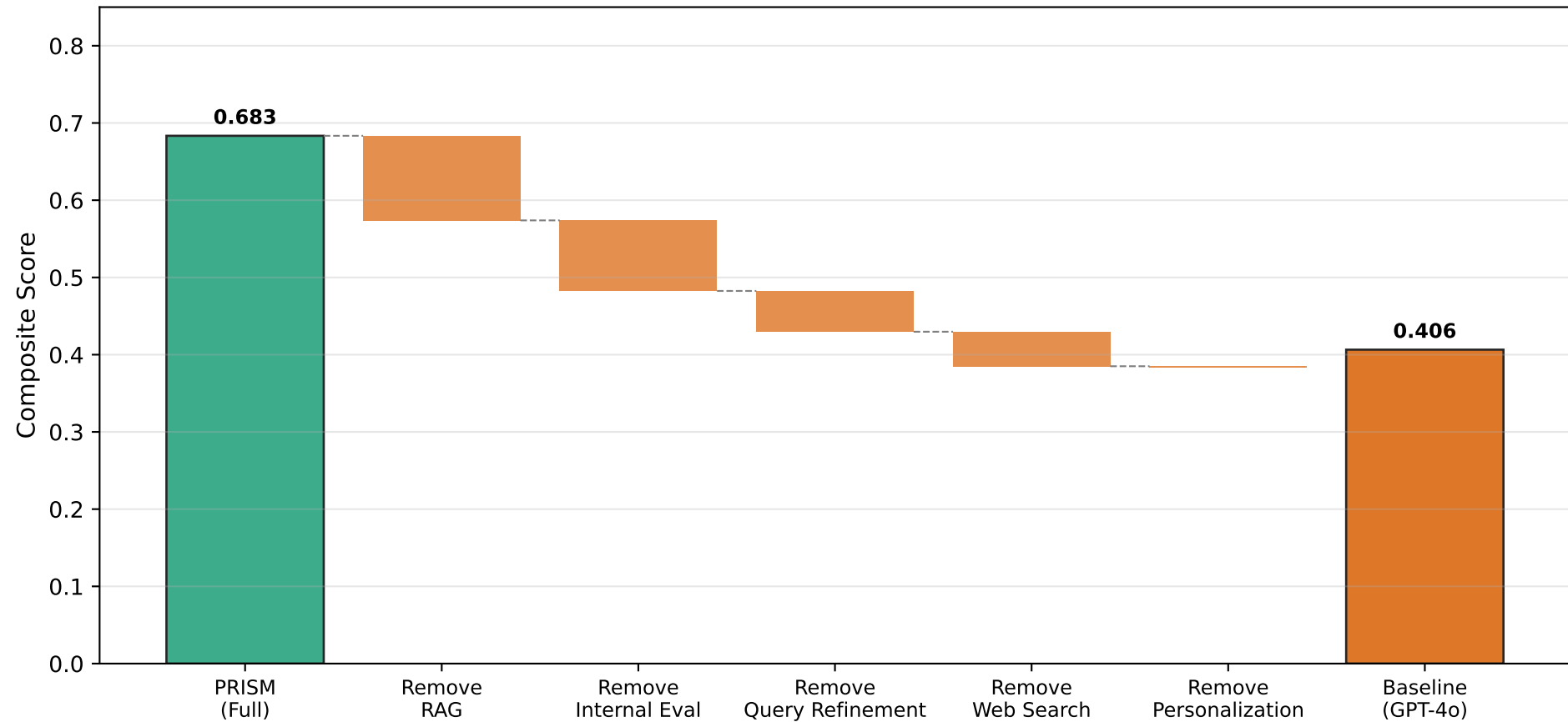
Ablation Waterfall: Impact of Removing Each PRISM Component
