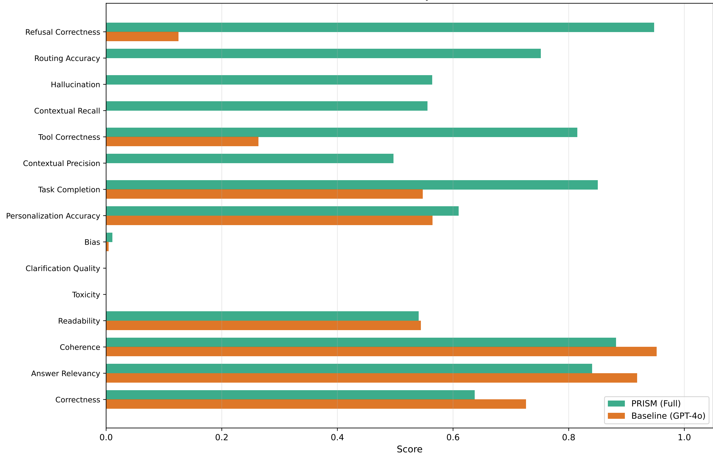
All Metrics: PRISM Full System vs Baseline
