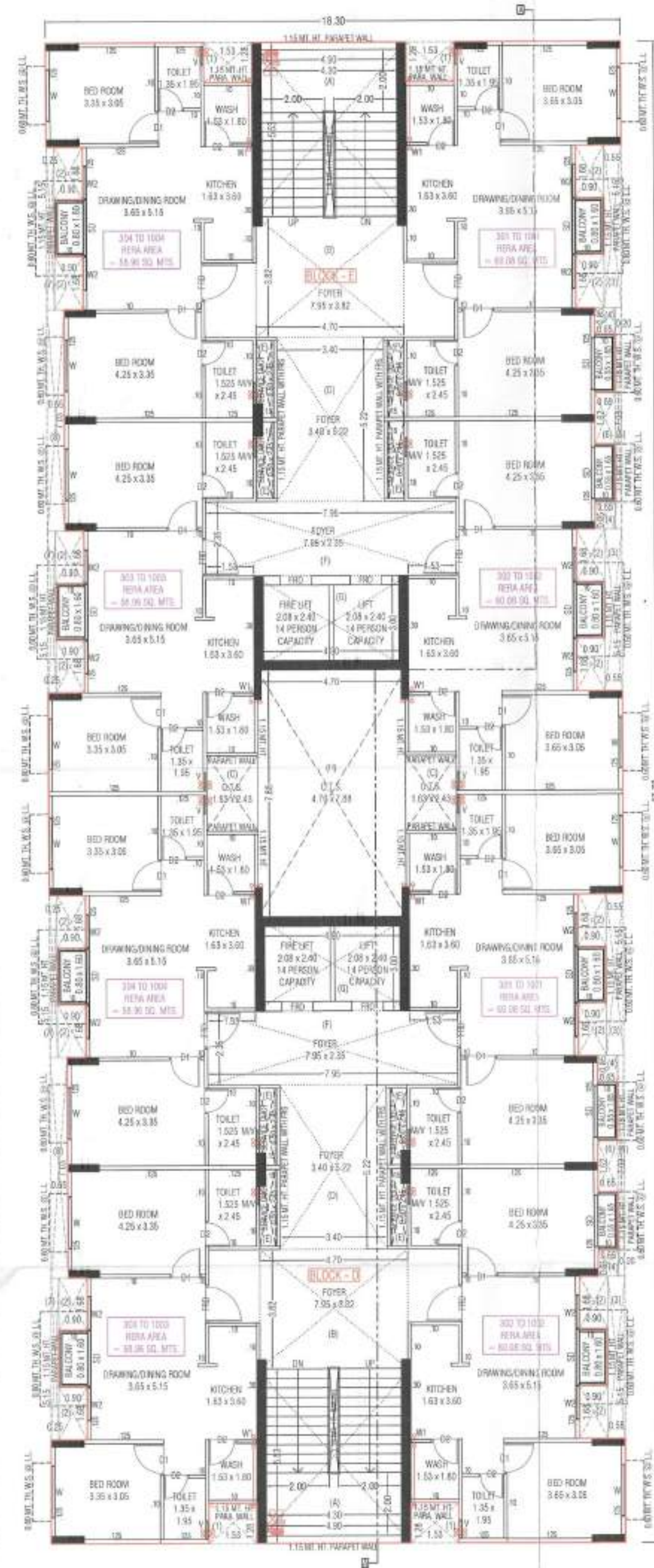
TYPICAL PLAN ( 3RD, 4TH, 6TH, 7TH, 9TH & 10TH FLOOR )
