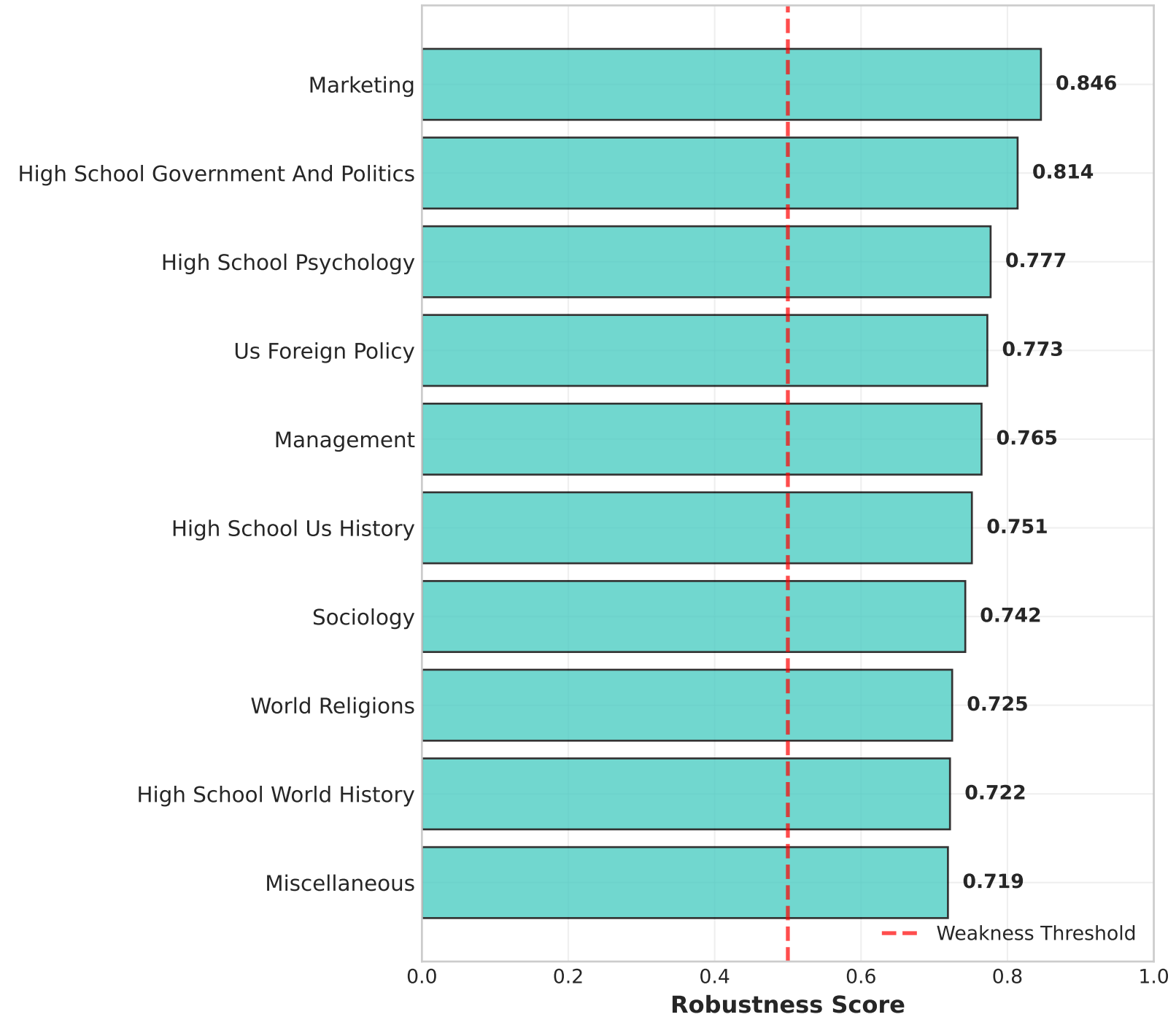
Non-Mathematical Domains (Top 10 Strongest)
