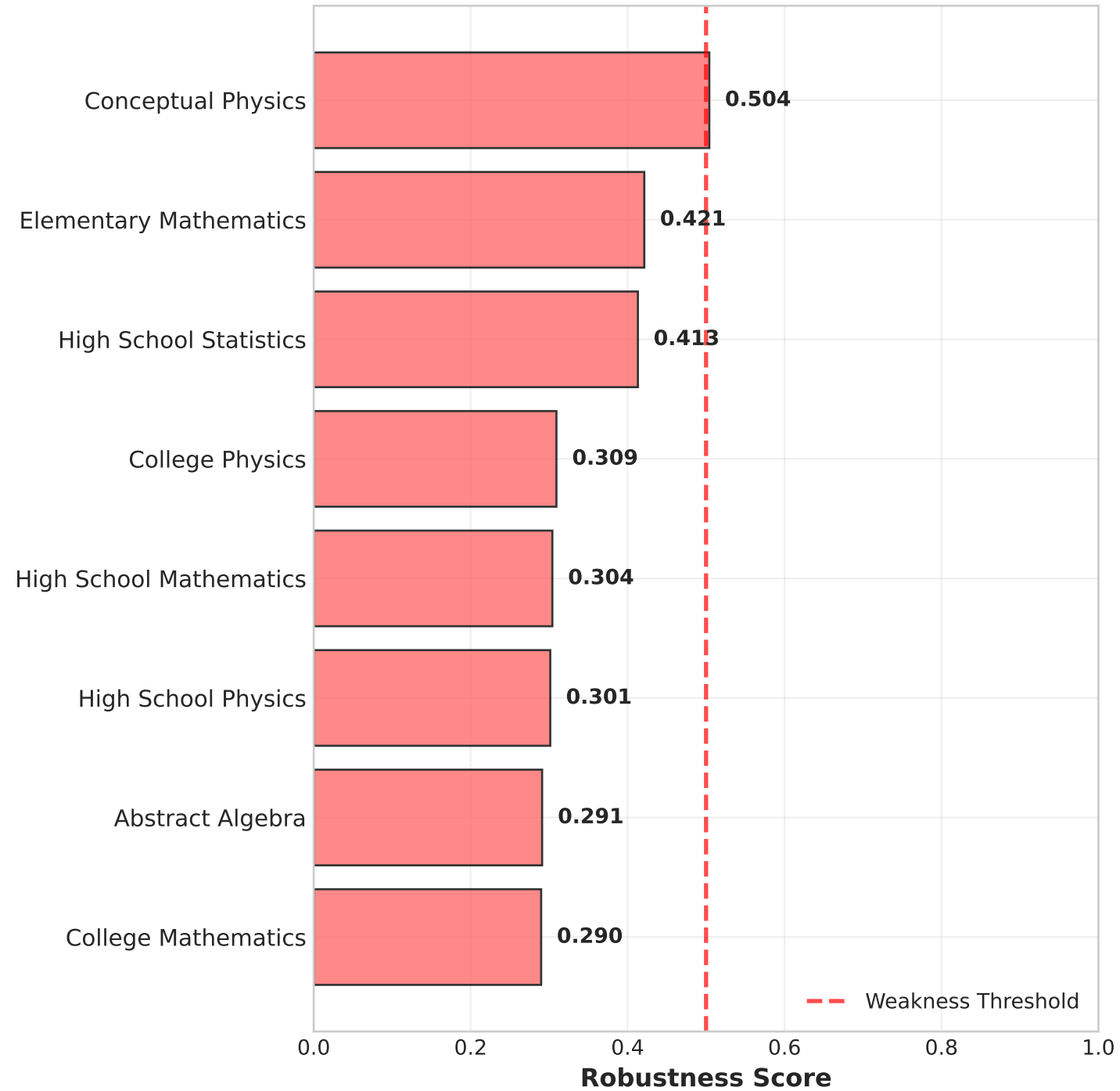
Mathematical Domains (Systematic Low Robustness)
