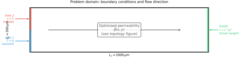
Figure 1: Problem domain with boundary conditions (schematic, not to scale). Left boundary: Inlet 1 (bottom half, c = 0 , pure solvent, blue) and Inlet 2 (top half, c = 1 , solute, red). Right boundary: outlet ( c = c^*(y) , target profile). Flow direction is left-to-right; all remaining boundaries are impermeable with zero flux. The optimised permeability distribution \bar{\rho}(\mathbf{x}) is shown in Figure 3.
