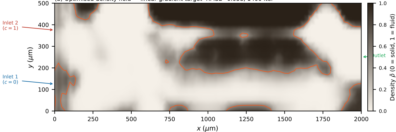
(a) Optimised density field — linear gradient target RMSE=0.058, 1400 iter
