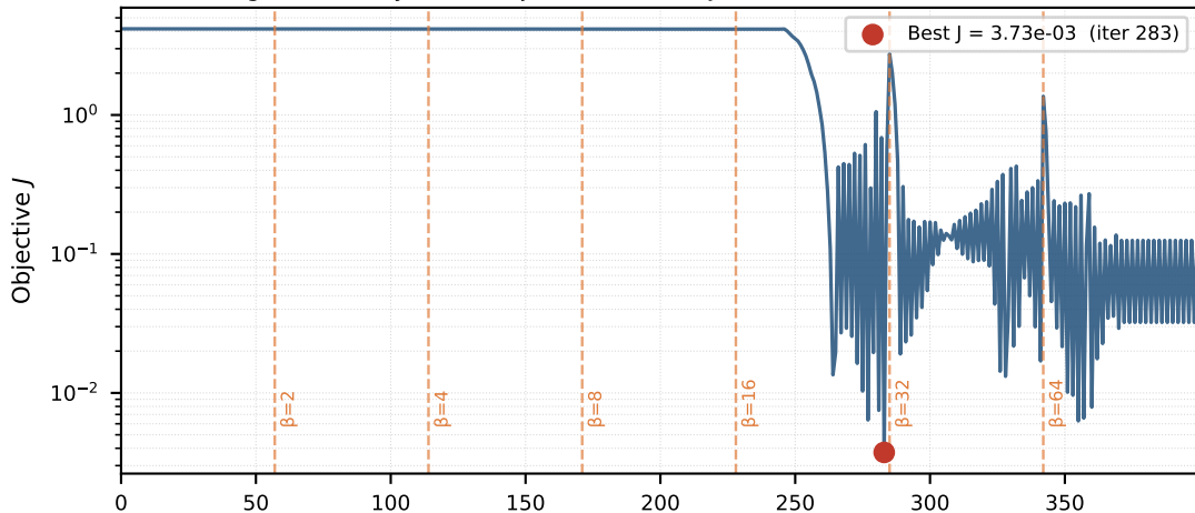
(a) Convergence history of the objective function J
